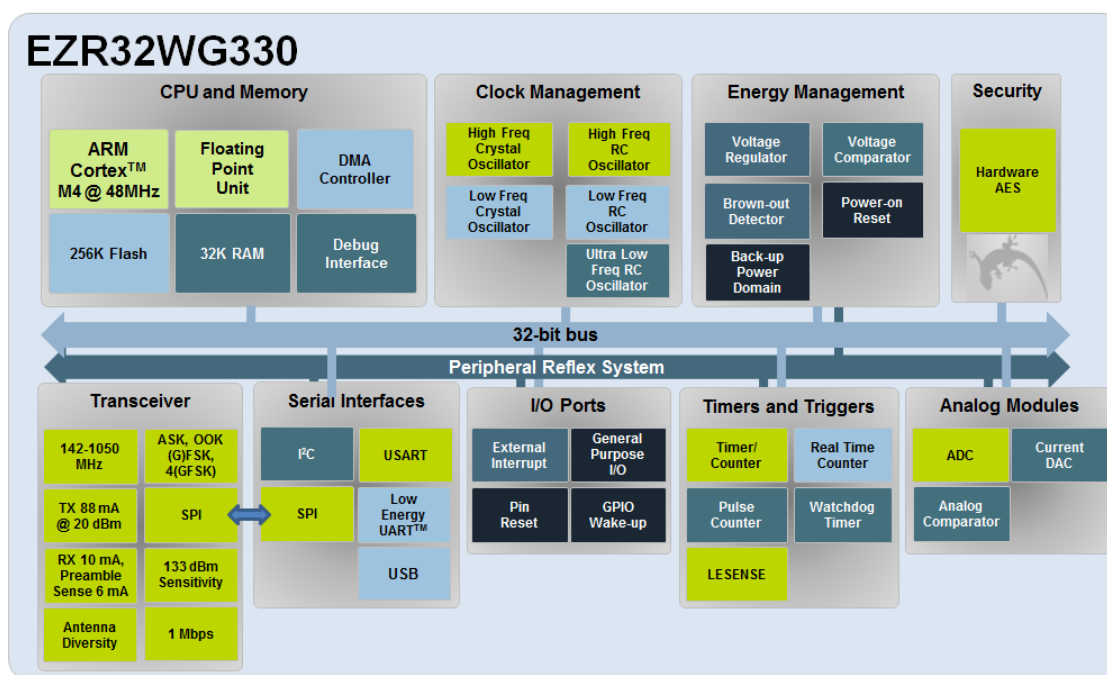
Figure 3.1. Block Diagram
