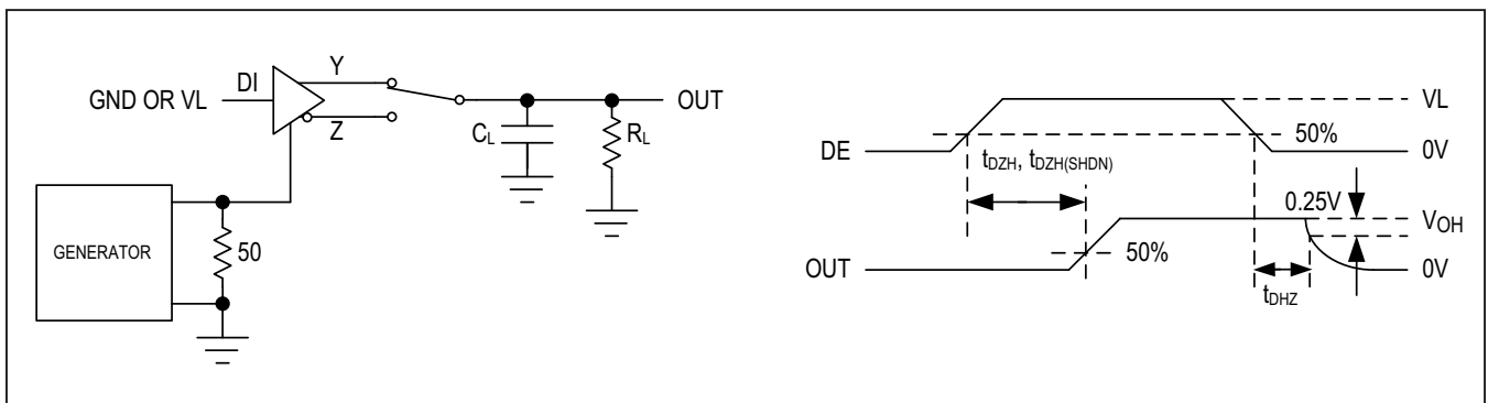
Figure 5. Driver Enable and Disable Times ( t_{DZH} , t_{DZH} )
