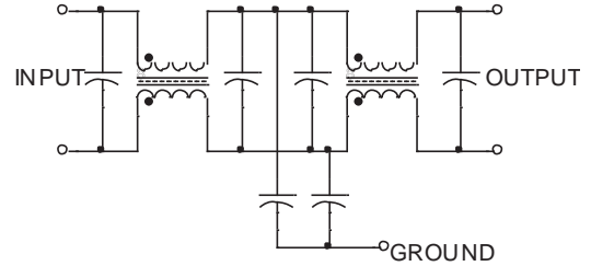
Figure 4. Internal Schematic
