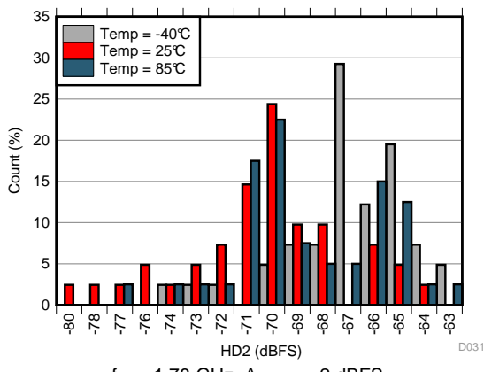
Figure 55. HD2 Histogram at AVDD19 = 1.8 V
