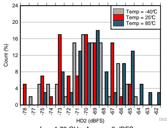
Figure 56. HD2 Histogram at AVDD19 = 1.9 V
