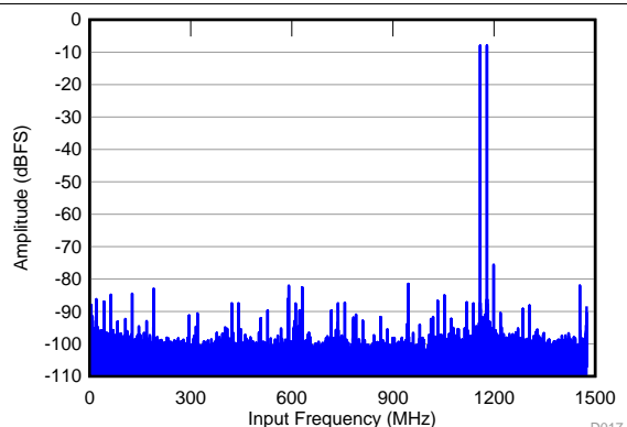
f_{IN1} = 1.77 \text{ GHz} , f_{IN2} = 1.79 \text{ GHz} , A_{IN} = -8 \text{ dBFS} , \text{IMD} = 75 \text{ dBFS}
