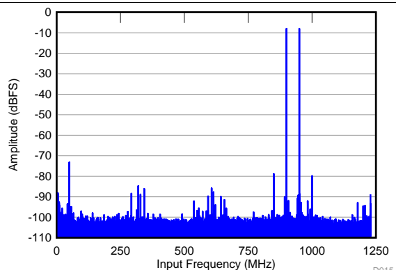
f_{IN1} = 900 \text{ MHz} , f_{IN2} = 950 \text{ MHz} , A_{IN} = -8 \text{ dBFS} , \text{IMD} = 78 \text{ dBFS}
