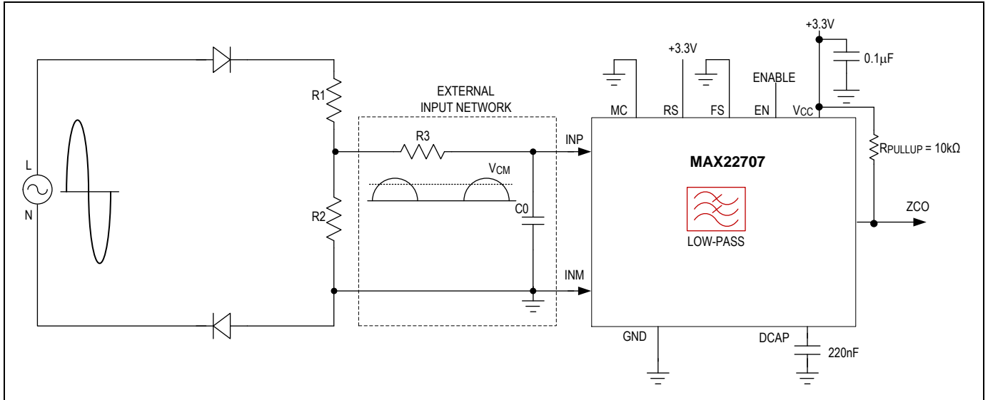
Figure 6. LPF for the Half-Rectified 50/60Hz Input
