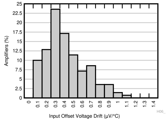
G = 10, 20, 30, 50 N = 140 \mu = 0.37\text{ }\mu\text{V}/^\circ\text{C} \sigma = 0.23\text{ }\mu\text{V}/^\circ\text{C}
