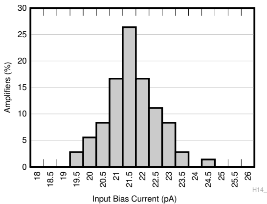
T_A = 85^\circ\text{C} N = 72 \mu = 22\text{ pA} \sigma = 0.95\text{ pA}
