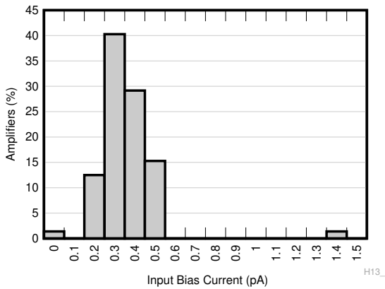
T_A = 25^\circ\text{C} N = 72 \mu = 0.40\text{ pA} \sigma = 0.15\text{ pA}
