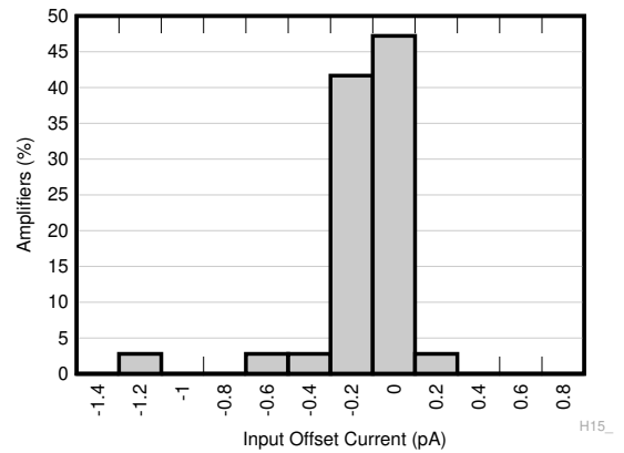
T_A = 25^\circ\text{C} N = 36 \mu = -0.03\text{ pA} \sigma = 0.23\text{ pA}
