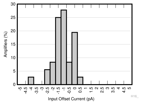
T_A = 85^\circ\text{C} N = 36 \mu = -1\text{ pA} \sigma = 1\text{ pA}
