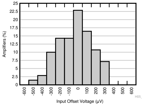
G = 10, 20, 30, 50 N = 140 \mu = 18\text{ }\mu\text{V} \sigma = 0.185\text{ mV}
