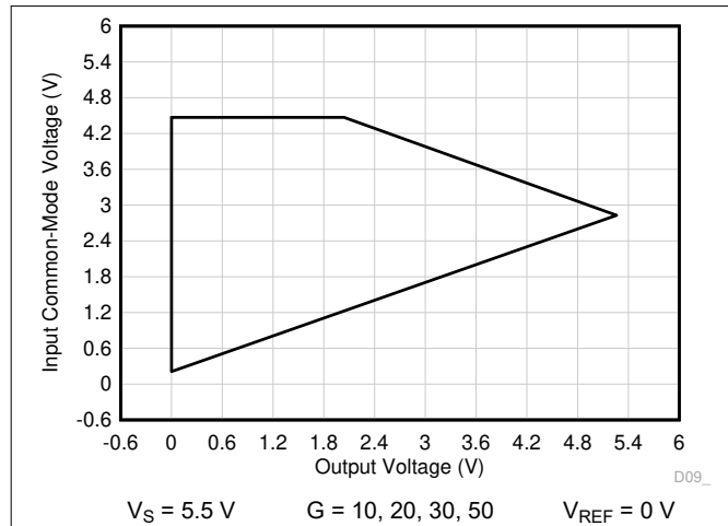
Figure 7-55. Input Common-Mode Voltage vs Output Voltage (High CMRR Region)
