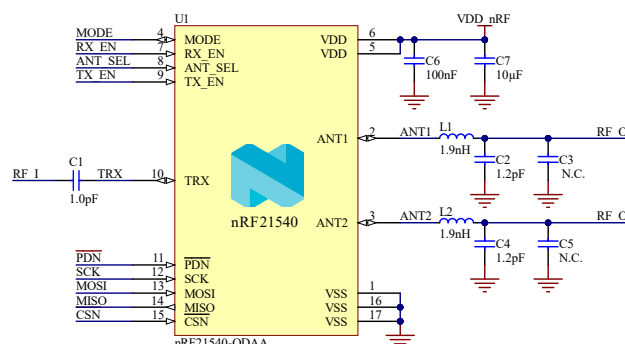
Figure 13: Reference circuitry schematic
