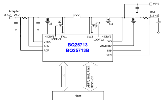
Application Diagram
