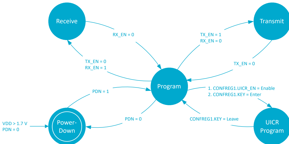
Figure 2: State diagram
