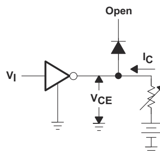
Figure 6-4. V_{I(on)} Test Circuit
