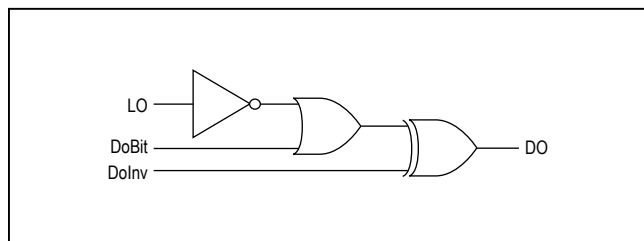
Figure 8. Equivalent DO Logic
