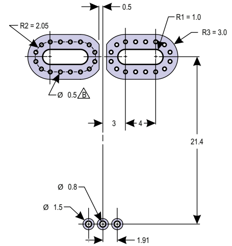
PCB Layout Reference View
