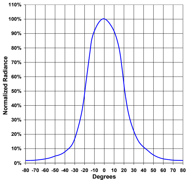
Beam Angle
