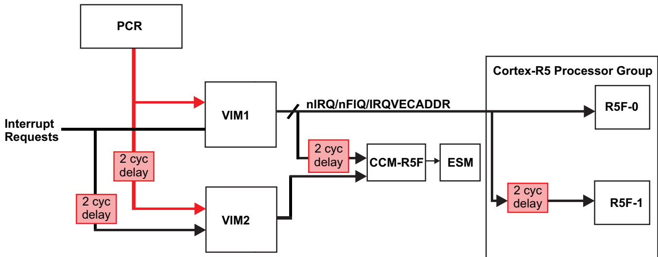
Figure 5-17. Interrupt Generation
