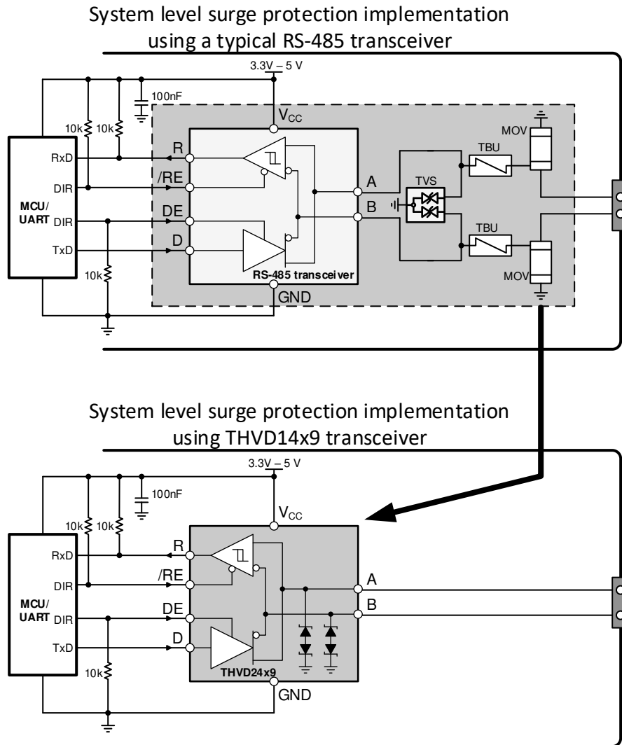
Figure 9-3. Implementation of System-Level Surge Protection Using THVD14x9(V)
