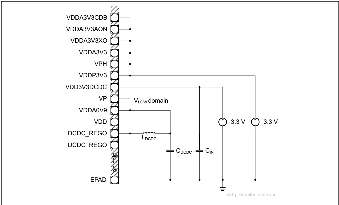
Figure 28 External Circuitry Using the Integrated DC/DC Converter
