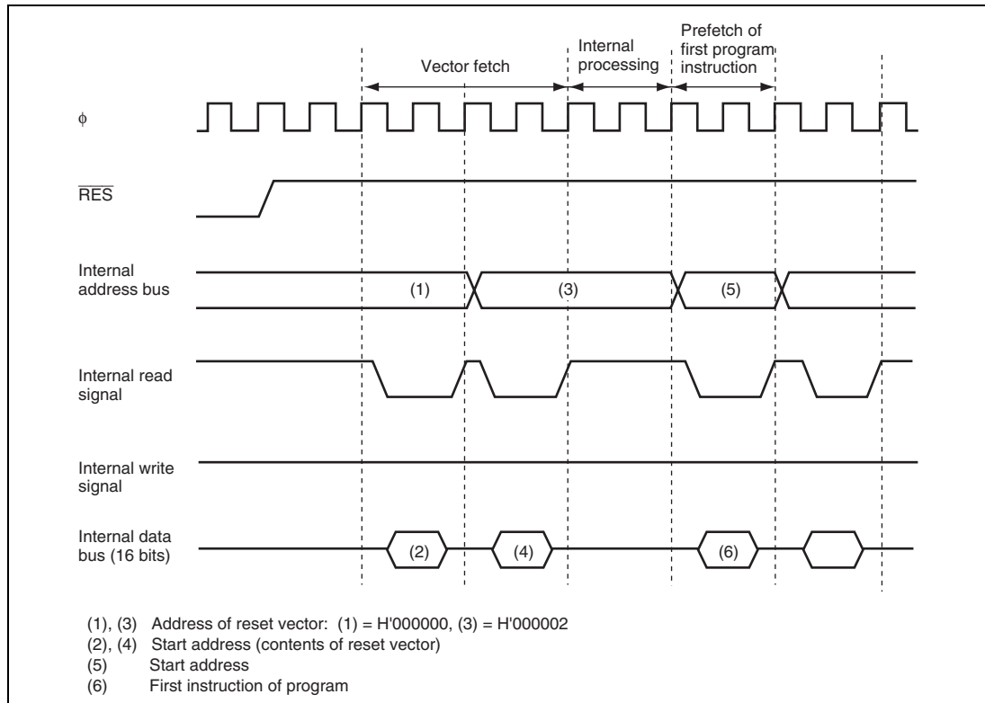
Figure 3.1 Reset Sequence
