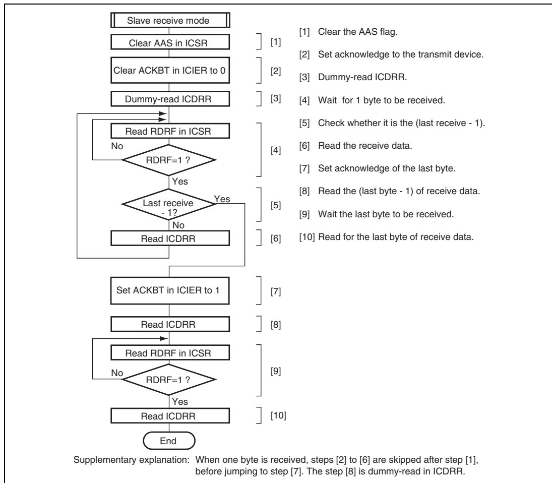
Figure 18.20 Sample Flowchart for Slave Receive Mode
