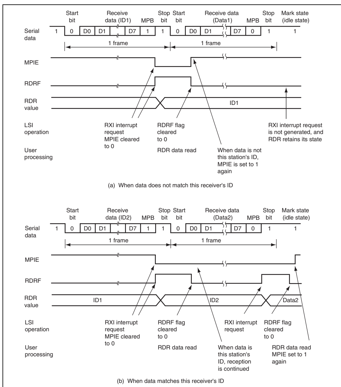
Figure 17.18 Example of SCI3 Reception Using Multiprocessor Format (Example with 8-Bit Data, Multiprocessor Bit, One Stop Bit)
