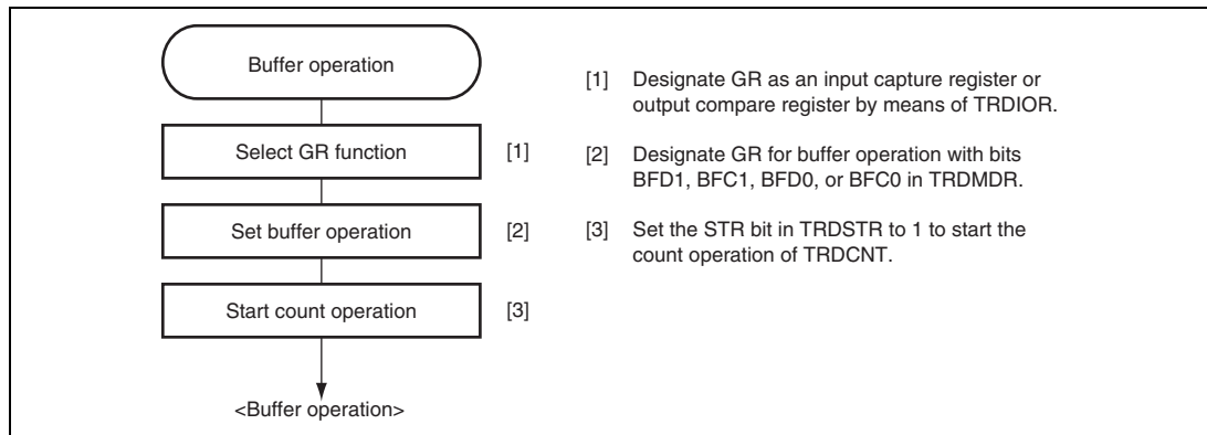
Figure 14.43 Example of Buffer Operation Setting Procedure
