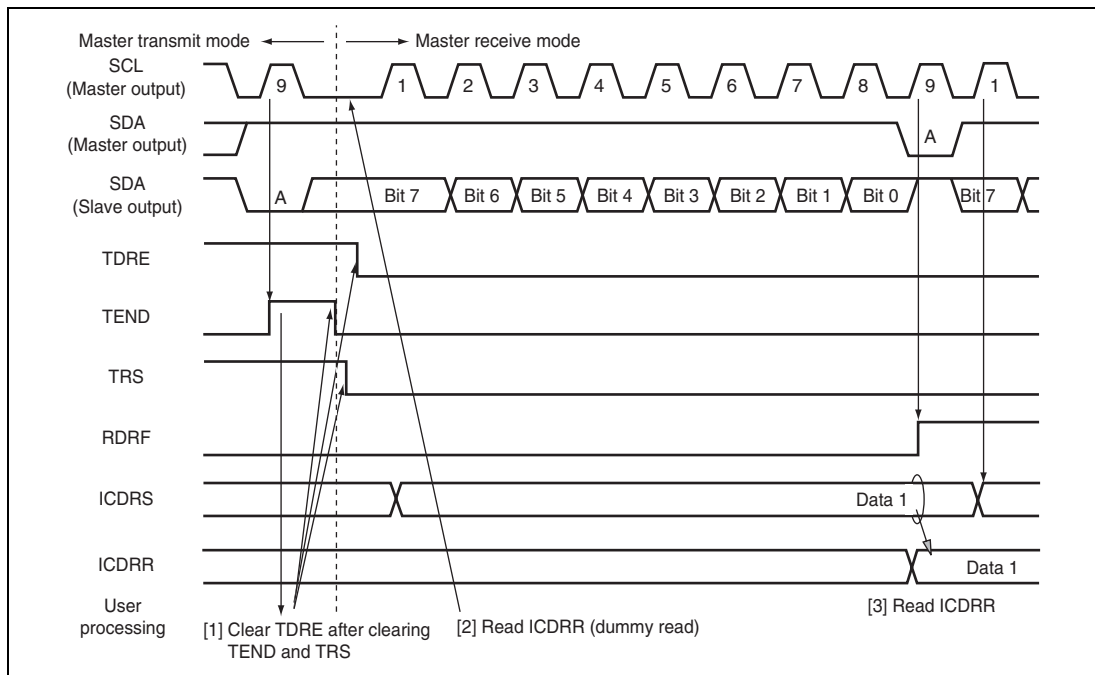
Figure 18.7 Master Receive Mode Operation Timing (1)
