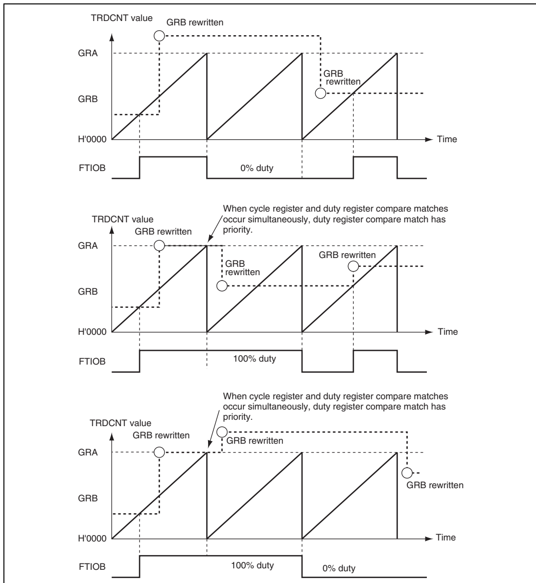
Figure 14.28 Example of PWM Mode Operation (4)
