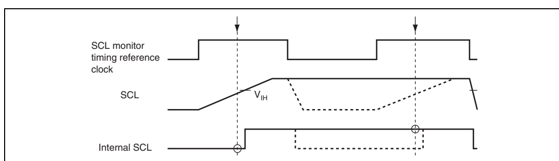
Figure 18.21 Timing of Bit Synchronous Circuit
