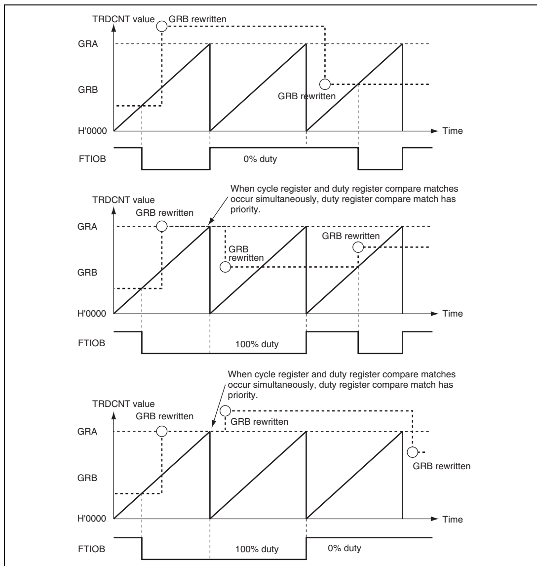
Figure 14.27 Example of PWM Mode Operation (3)
