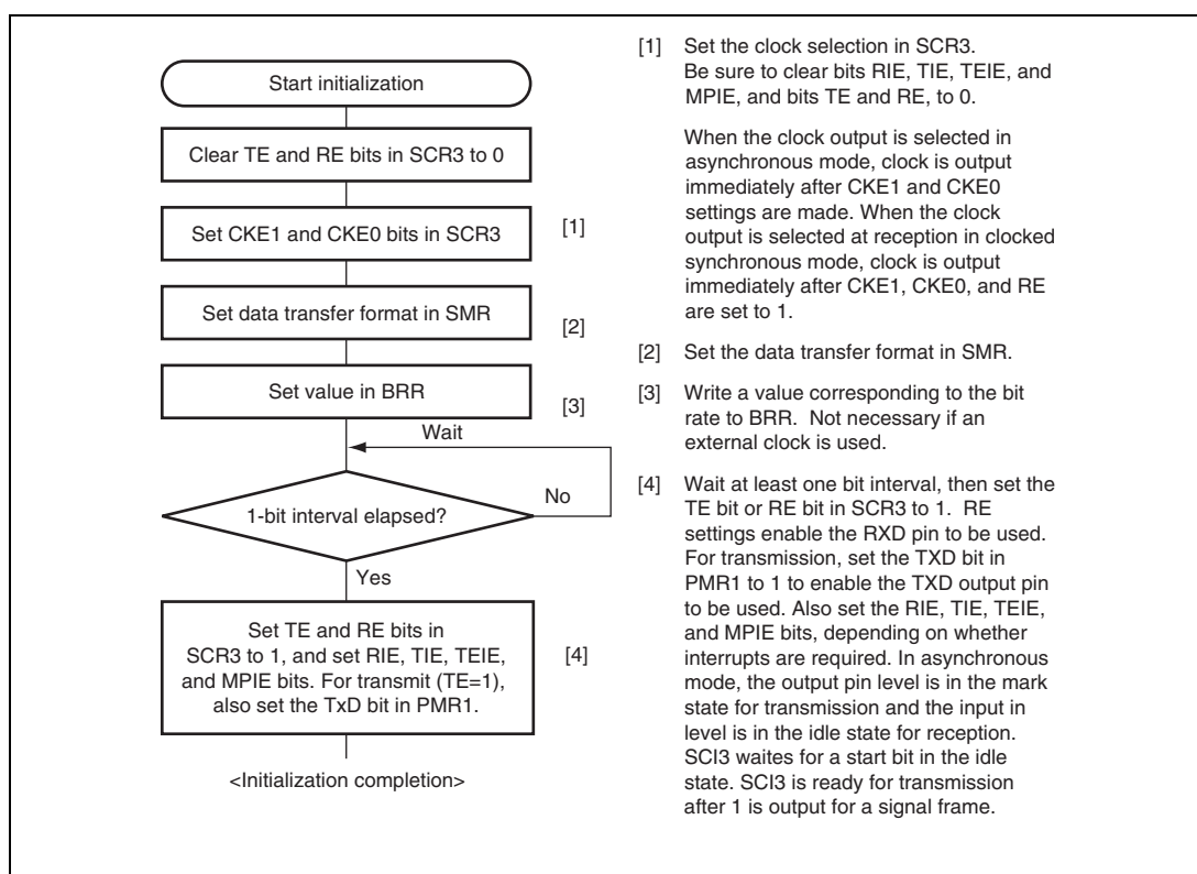
Figure 17.4 Sample SCI3 Initialization Flowchart
