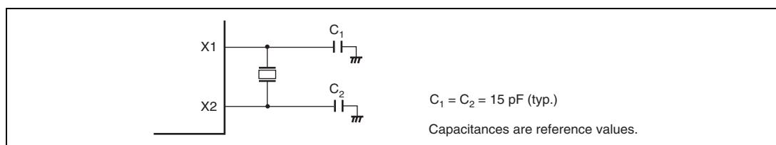
Figure 5.15 Typical Connection to 32.768-kHz Crystal Resonator
