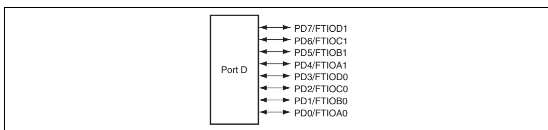
Figure 9.8 Port D Pin Configuration
