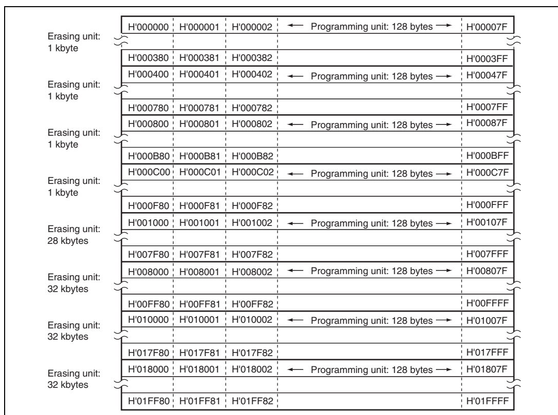
Figure 7.1 Block Configuration of Flash Memory
