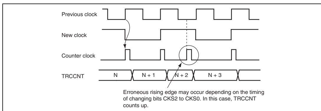
Figure 13.34 Internal Clock Switching and TRCCNT Operation
