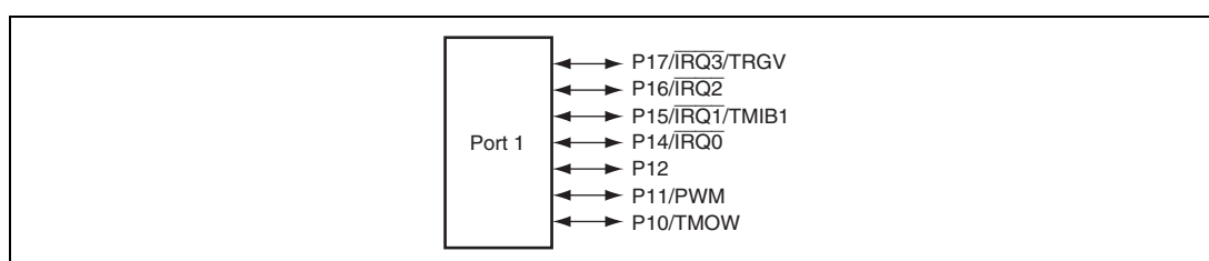
Figure 9.1 Port 1 Pin Configuration
