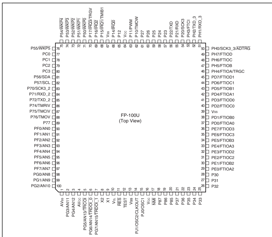
Figure 1.3 Pin Assignments (FP-100U)
