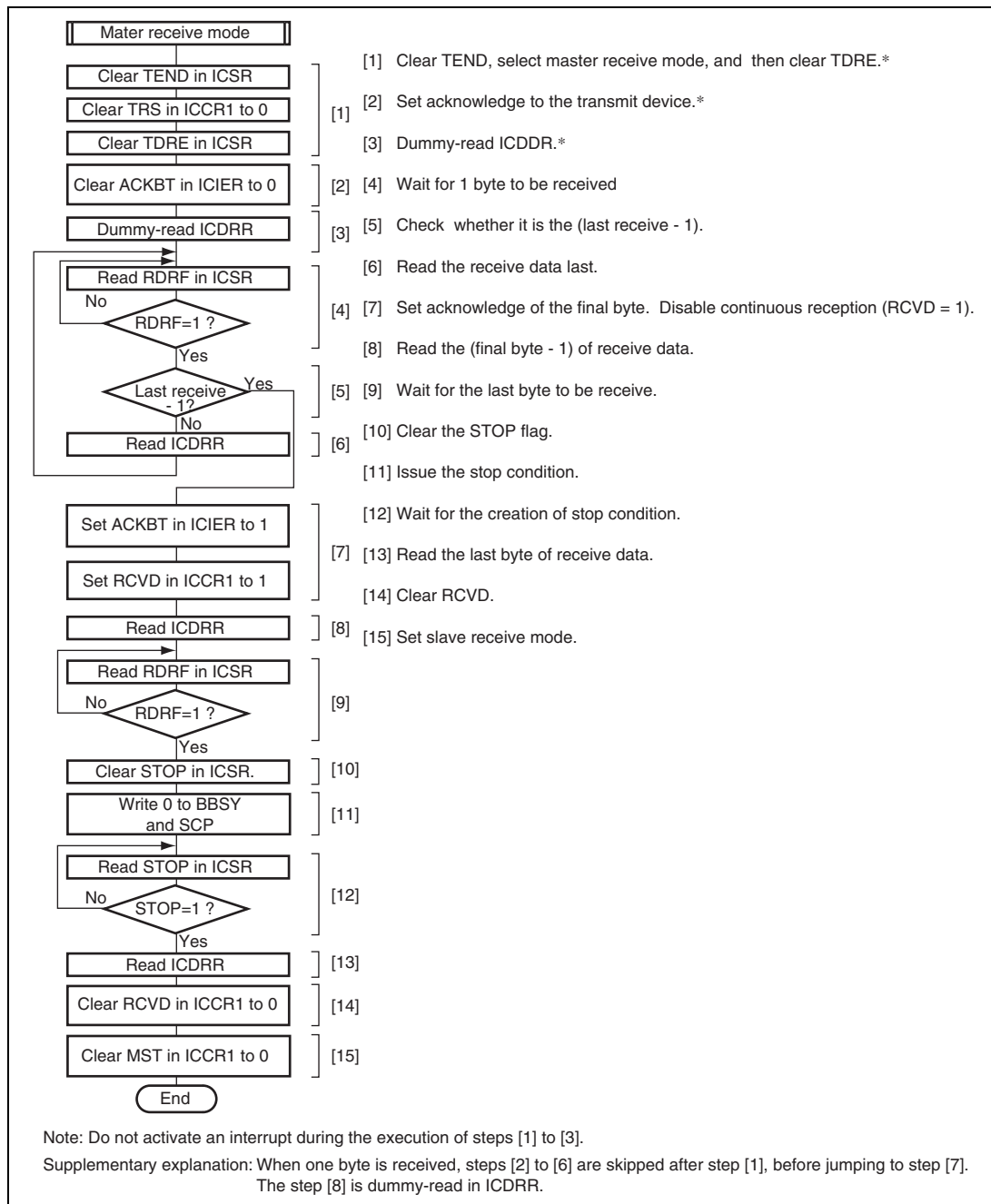
Figure 18.18 Sample Flowchart for Master Receive Mode
