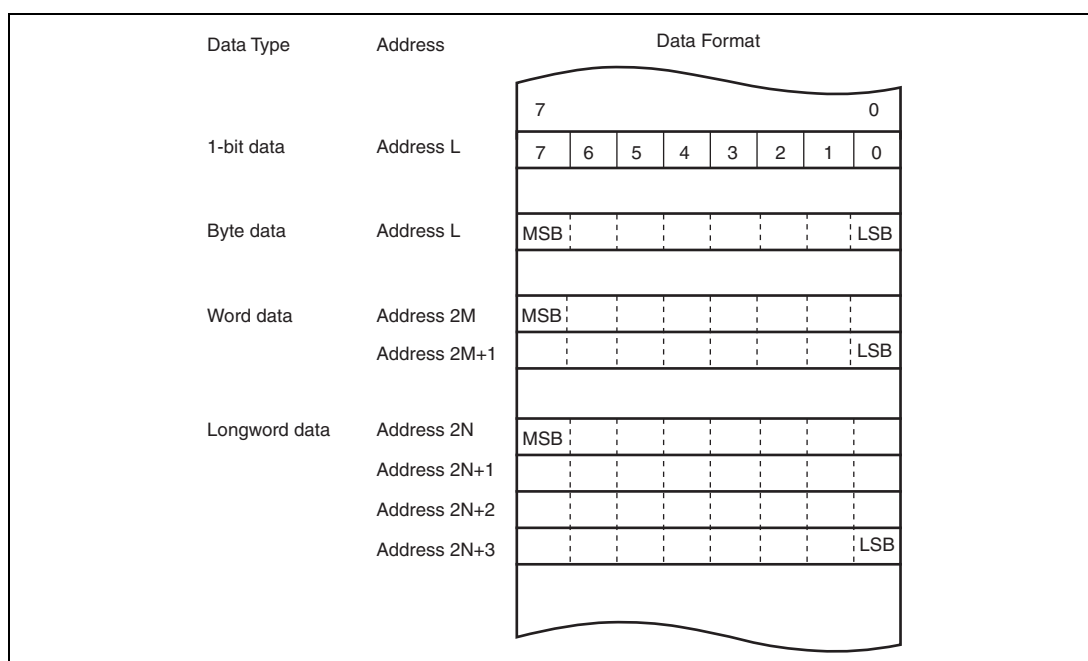
Figure 2.6 Memory Data Formats
