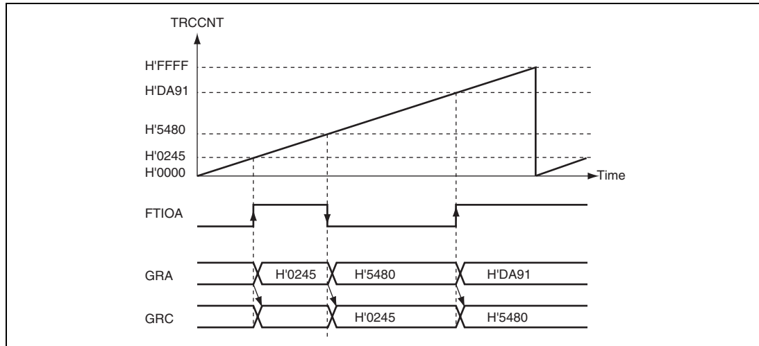
Figure 13.8 Buffer Operation Example (Input Capture)
