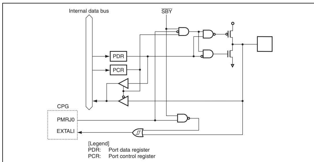
Figure B.34 Port J Block Diagram (PJ0)
