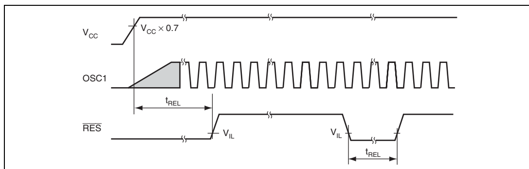
Figure 23.2 \overline{RES} Low Width Timing
