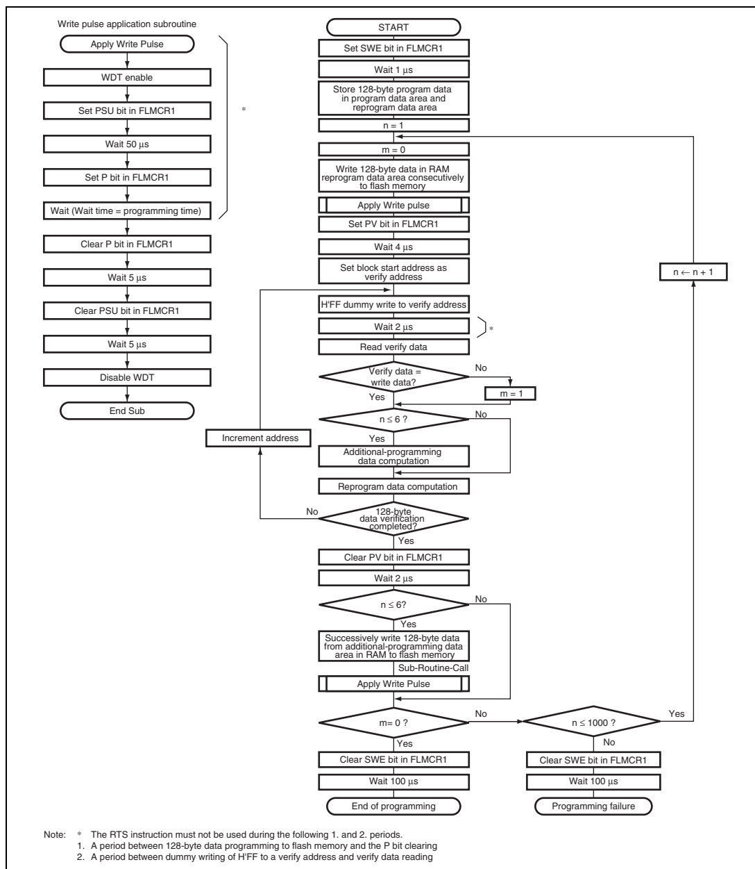
Figure 7.3 Programming/Program-Verify Flowchart
