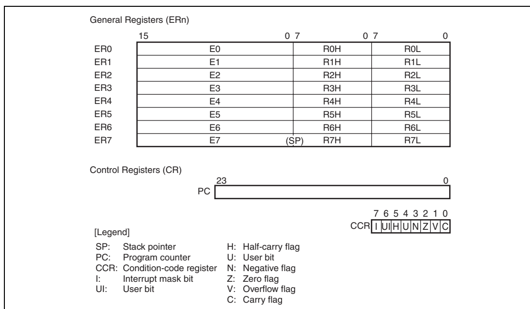
Figure 2.2 CPU Registers
