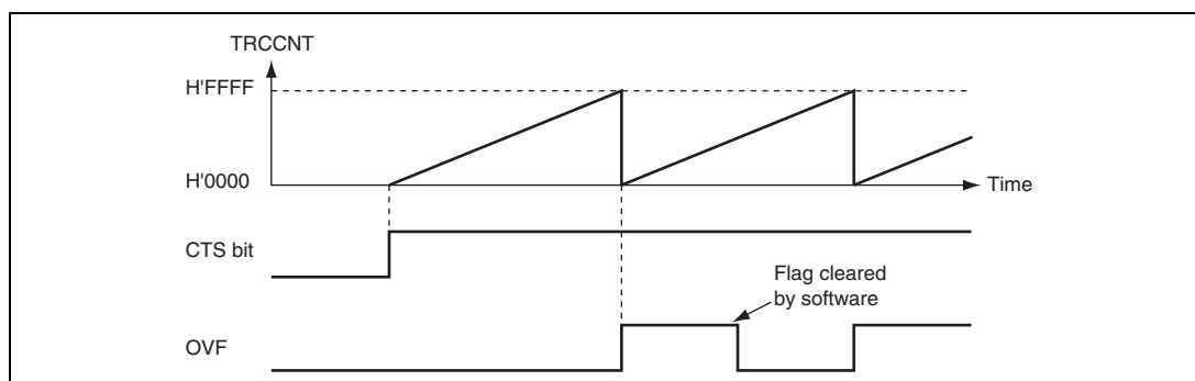
Figure 13.2 Free-Running Counter Operation
