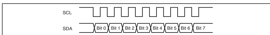
Figure 18.13 Clocked Synchronous Serial Transfer Format
