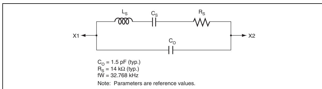
Figure 5.16 Equivalent Circuit of 32.768-kHz Crystal Resonator
