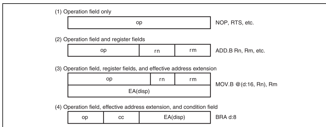
Figure 2.7 Instruction Formats
