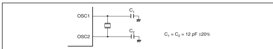
Figure 5.10 Example of Connection to Crystal Resonator
