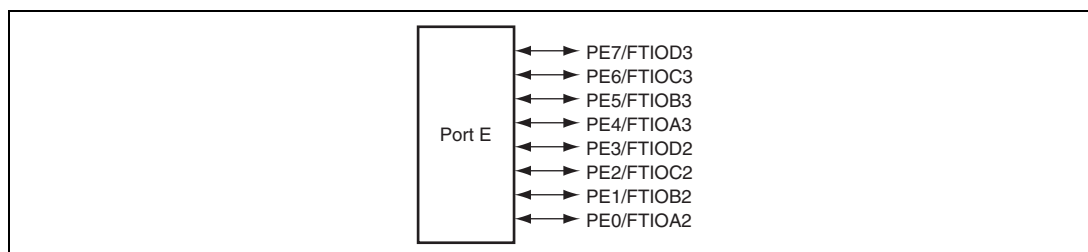
Figure 9.9 Port E Pin Configuration
