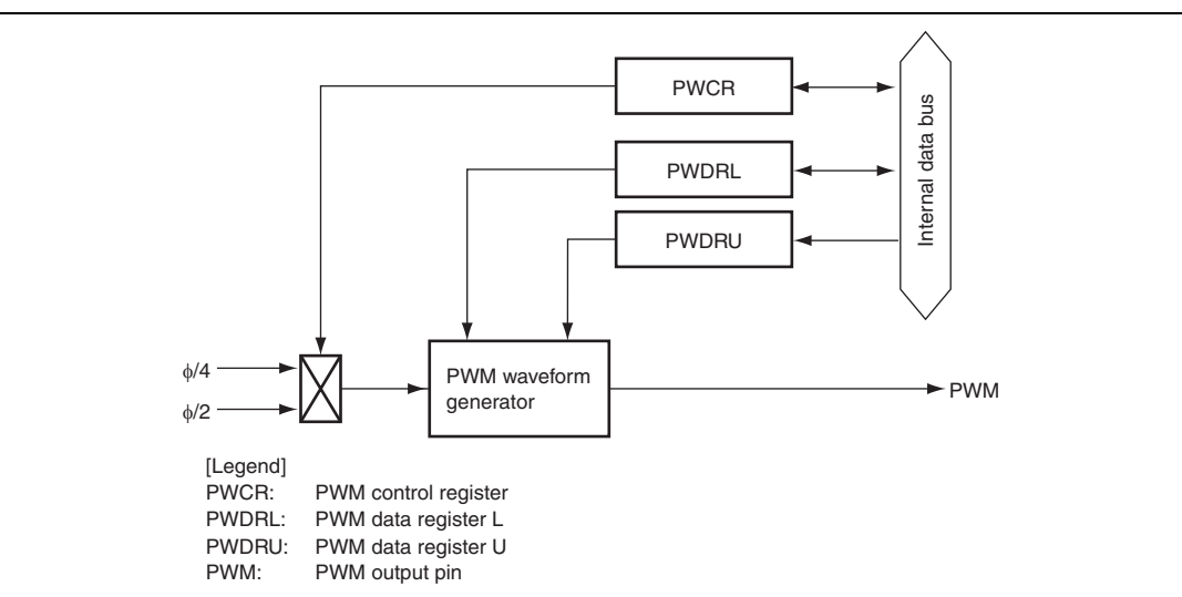
Figure 16.1 Block Diagram of 14-Bit PWM
