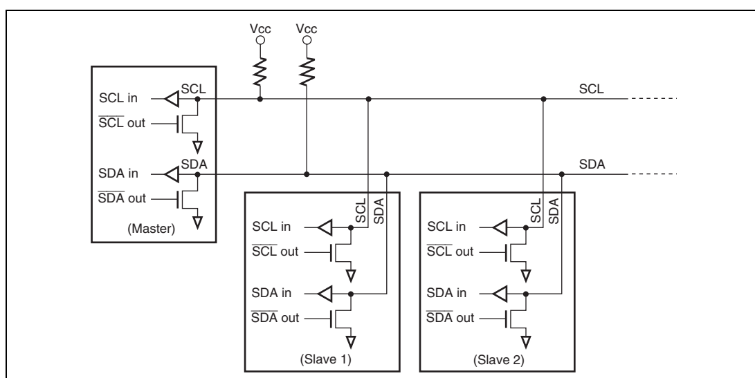
Figure 18.2 External Circuit Connections of I/O Pins
