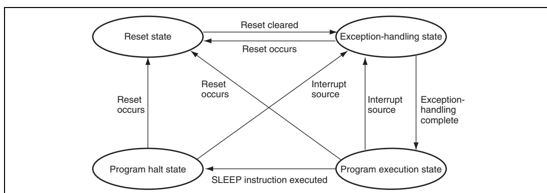
Figure 2.12 State Transitions
