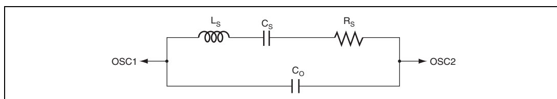
Figure 5.11 Equivalent Circuit of Crystal Resonator
