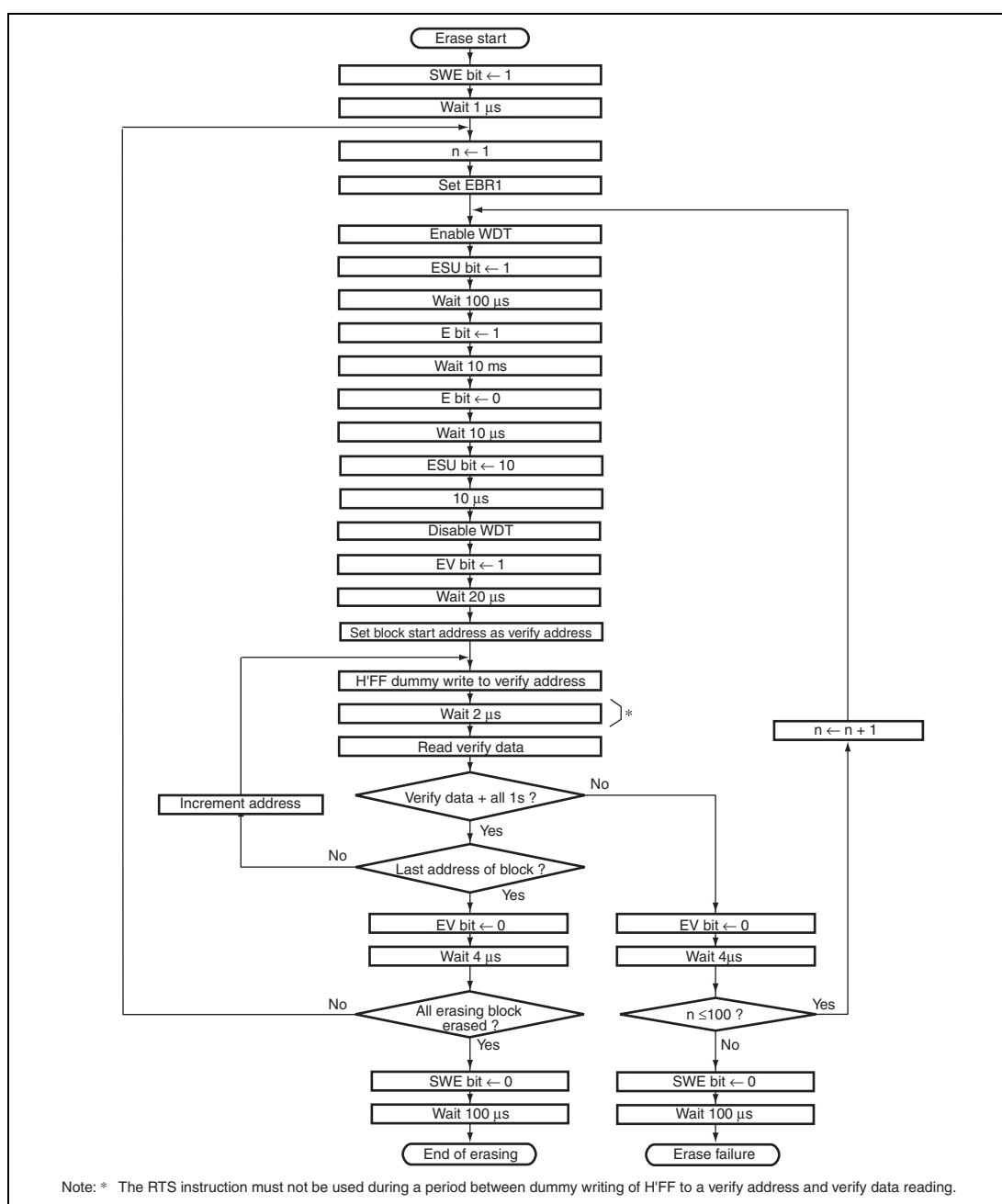
Figure 7.4 Erasure/Erase-Verify Flowchart
