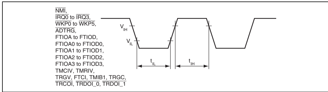
Figure 23.3 Input Timing
