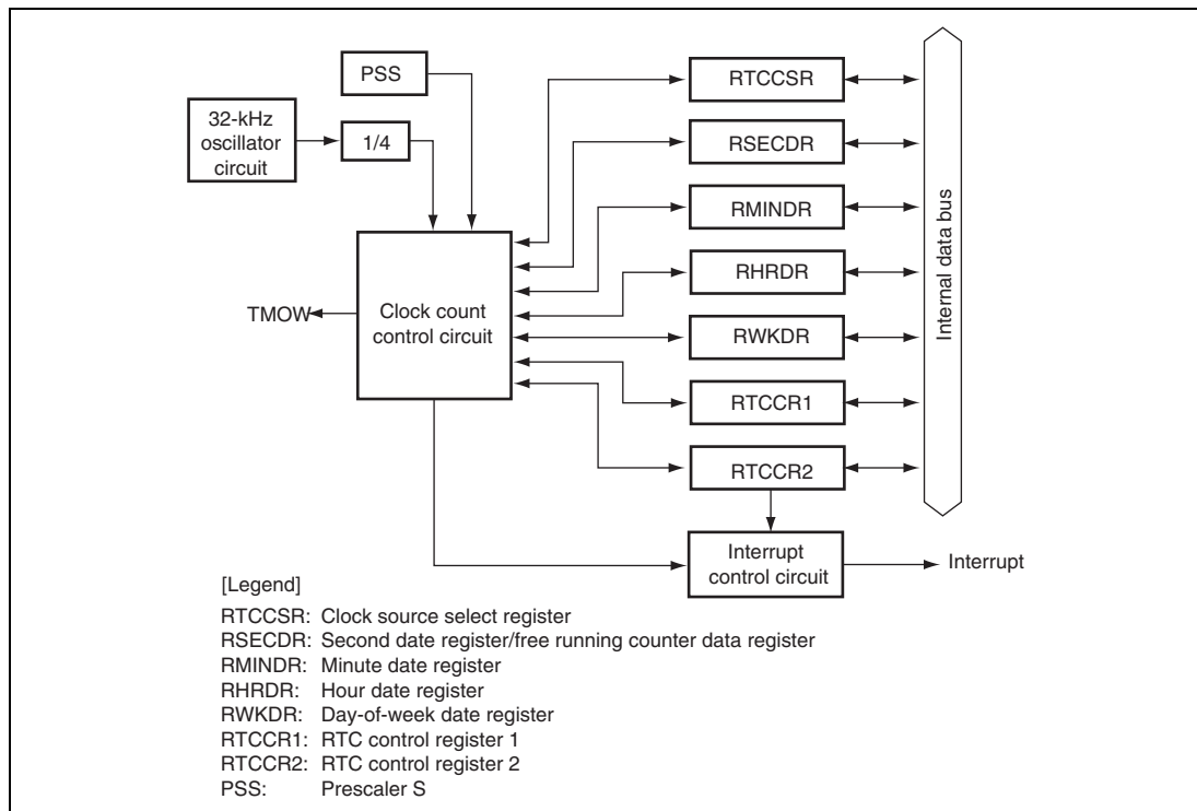
Figure 10.1 Block Diagram of RTC
