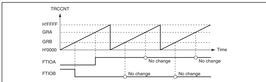
Figure 13.4 0 and 1 Output Example (TOA = 0, TOB = 1)
