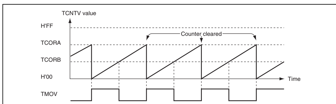
Figure 12.9 Pulse Output Example
