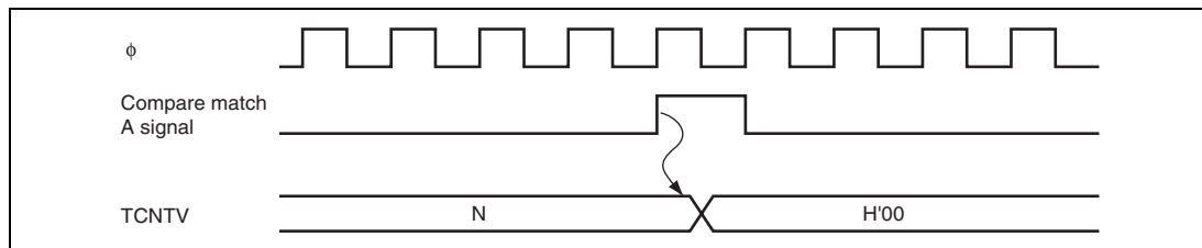
Figure 12.7 Clear Timing by Compare Match
