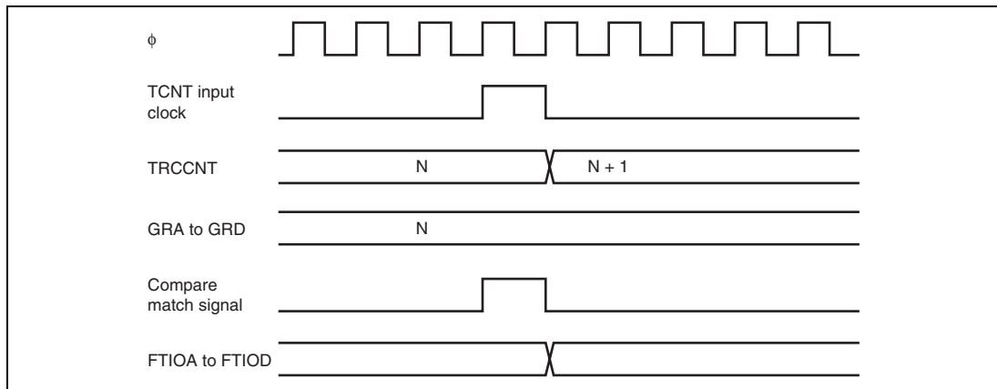
Figure 13.25 Output Compare Output Timing
