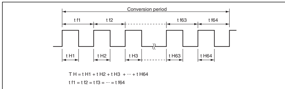
Figure 16.2 Waveform Output by 14-Bit PWM
