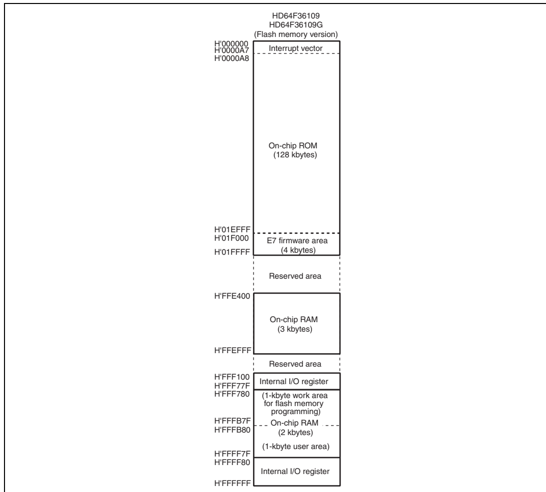
Figure 2.1 Memory Map
