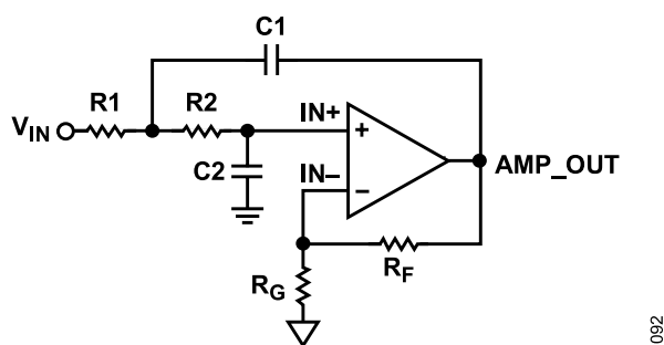
Figure 87. Schematic of a Second-Order, Low-Pass Active Filter
