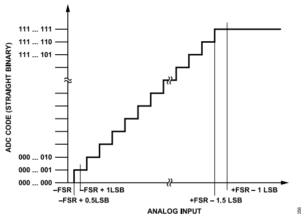
Figure 53. ADC Ideal Transfer Function
