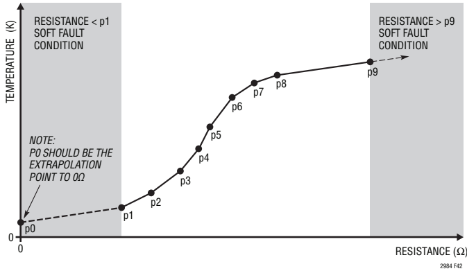
Figure 42. Custom RTD Example ( \Omega vs Kelvin )
