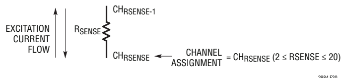
Figure 20. Sense Resistor Channel Assignment Convention for 4-Wire RTDs with Rotation
