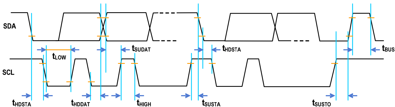
Figure 14. Timing Diagram
