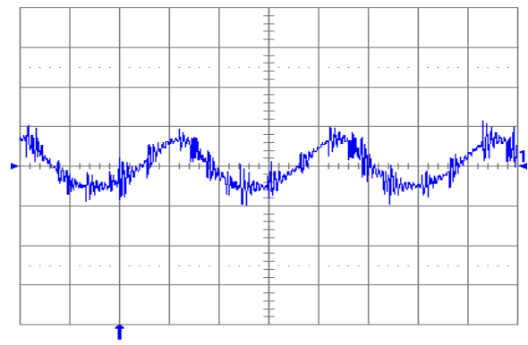
Fig. 3.3V.6: Output voltage ripple (20 mV/div.) at full rated load current into a resistive load with external capacitance 47\ \mu\text{F} ceramic + 1\ \mu\text{F} ceramic, and V_{in} = 5\text{ V} for V_{out} = 3.3\text{ V} . Time scale: 2 \mu\text{s} /div.
