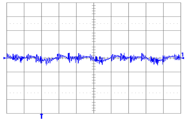
Fig. 0.7525V.6: Output voltage ripple (20 mV/div.) at full rated load current into a resistive load with external capacitance 47\text{ }\mu\text{F} ceramic + 1\text{ }\mu\text{F} ceramic, and V_{in} = 5\text{ V} for V_{out} = 0.7525\text{ V} . Time scale: 2 \mu\text{s} /div.
