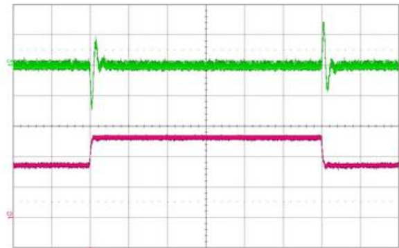
Figure 35. Output voltage response to load current step-change (17.5 A – 26.25 A – 17.5 A) at V_{in} = 48\text{ V} . Top trace: output voltage (200 mV/div.). Bottom trace: load current (10 A/div.). Current slew rate: 1 A/ \mu\text{s} . C_o = 1\ \mu\text{F} ceramic + 10 \mu\text{F} tantalum. Time scale: 200 \mu\text{s} /div.
