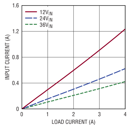
Input vs Load Current, V_{OUT} = 3.3\text{V} \text{BIAS} = 5\text{V} , Burst Mode
