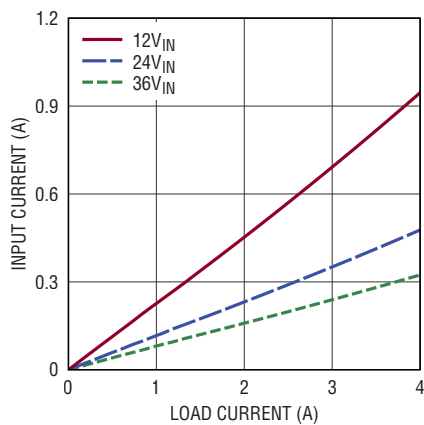
Input vs Load Current, V_{OUT} = 2.5\text{V} \text{BIAS} = 5\text{V} , Burst Mode
