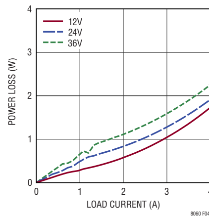
Figure 4. Power Loss Curves
