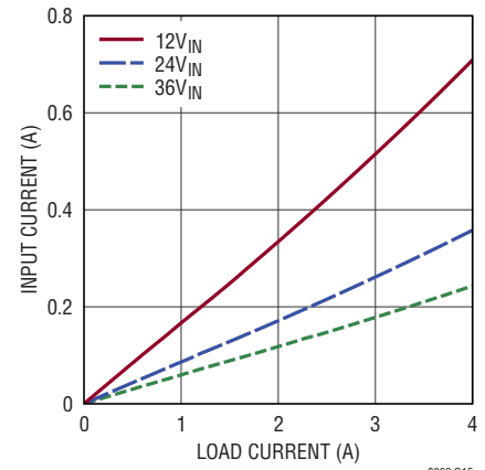
Input vs Load Current, V_{OUT} = 1.8\text{V} \text{BIAS} = 5\text{V} , Burst Mode
