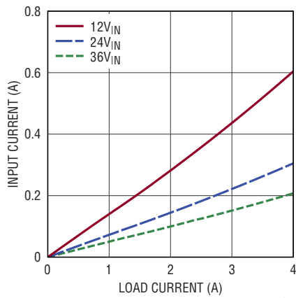
Input vs Load Current, V_{OUT} = 1.5\text{V} \text{BIAS} = 5\text{V} , Burst Mode
