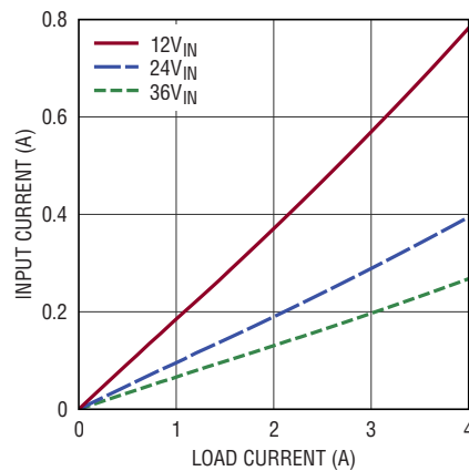
Input vs Load Current, V_{OUT} = 2\text{V} \text{BIAS} = 5\text{V} , Burst Mode
