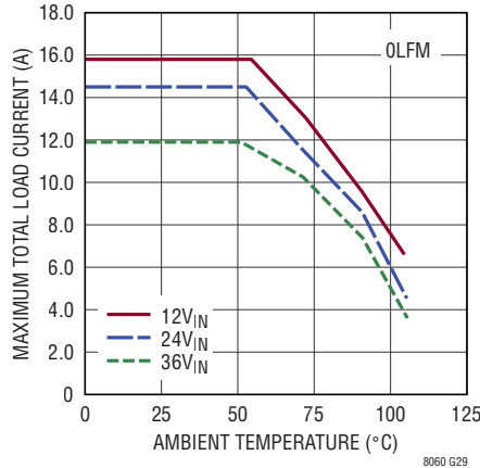
Derating, V_{OUT} = 8\text{V} BIAS = 5V, DC2820A Demo Board T_J = 120^\circ\text{C} , Burst Mode All Channels at Same Load
