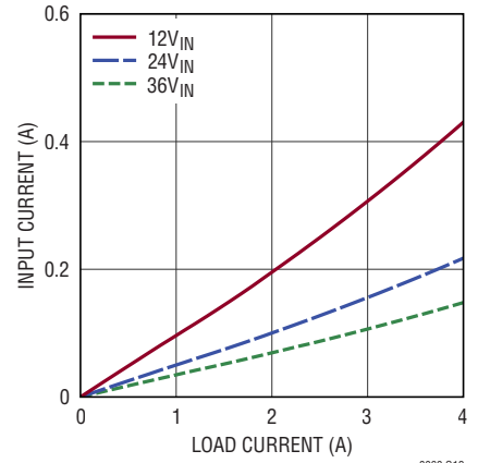
Input vs Load Current, V_{OUT} = 1\text{V} \text{BIAS} = 5\text{V} , Burst Mode
