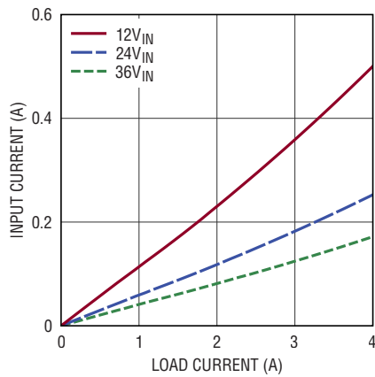
Input vs Load Current, V_{OUT} = 1.2\text{V} \text{BIAS} = 5\text{V} , Burst Mode
