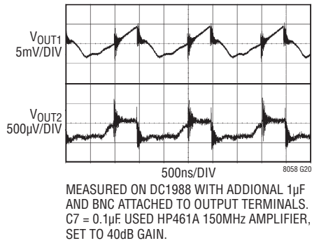
Typical Output Ripple 100mA Output Current, V_{IN} = 12V
