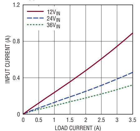
Input vs Load Current, V_{OUT} = 2.5\text{V}
