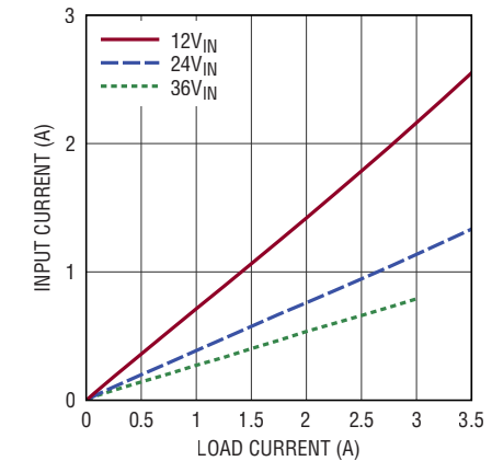
Input vs Load Current, V_{OUT} = 8\text{V}
