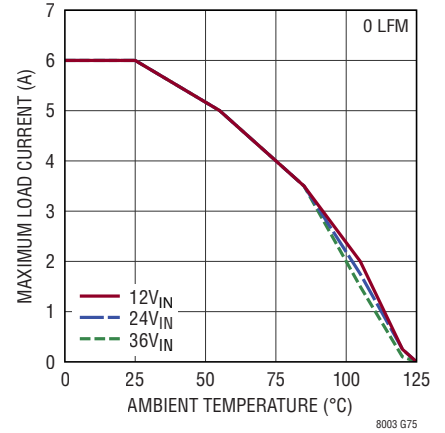
Derating, I-Grade, V_{OUT} = 2\text{V} , BIAS = 5V, DC2416A Demo Board
