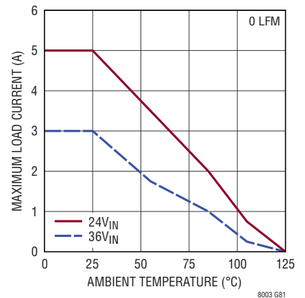
Derating, I-Grade, V_{OUT} = 15\text{V} , BIAS = 5V, DC2416A Demo Board
