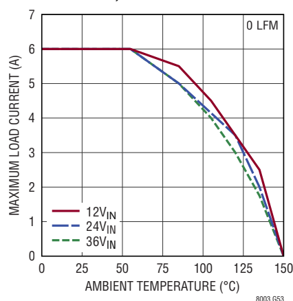
Derating, H-Grade, V_{OUT} = 0.97\text{V} , \text{BIAS} = 5\text{V} , DC2416A Demo Board
