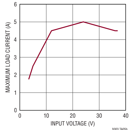
Maximum Load Current vs V_{IN} . BIAS Tied to LTM8003 GND
