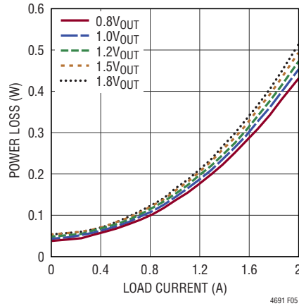
Figure 5. Power Loss at 3.3V IN , Per Channel
