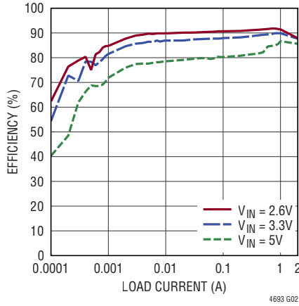
1.8V OUT Efficiency, 1MHz, Burst Mode Operation
