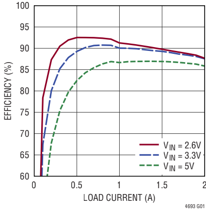
1.8V OUT Efficiency, 1MHz, CCM
