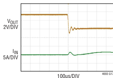
Short-Circuit with No Load
