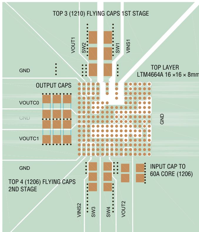
Figure 45. Recommended PCB Layout Package Top and Bottom View
