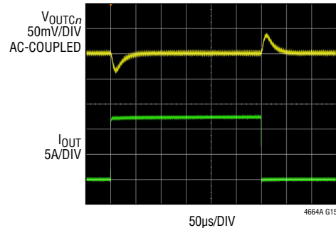
V_{OUTCn} (1.5V) Load Transient
