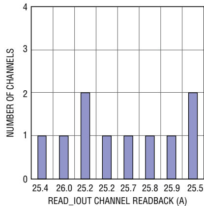
READ_IOUT of 16 LTM4664A Channels 12VIN, 1VOUT, TJ = -40°C, IOUTn = 25A, System Having Reached Thermally Steady-State Condition, No Airflow
