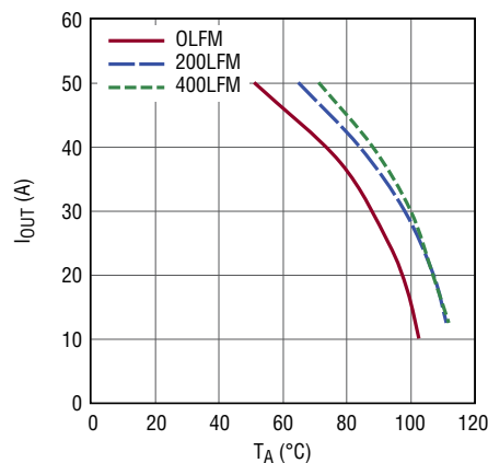
Figure 43. LTM4664A 48V IN 1.5V OUT 350kHz Derating Curve No Heat Sink
