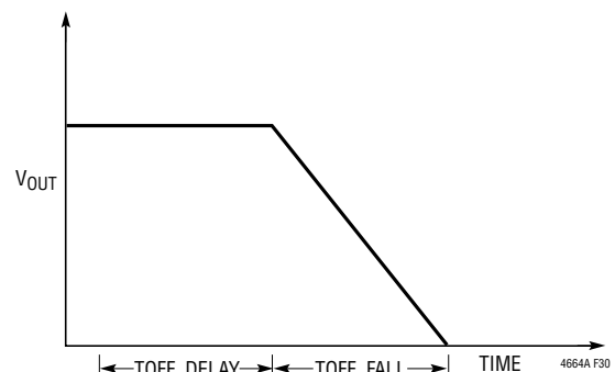
Figure 30. TOFF_DELAY and TOFF_FALL
