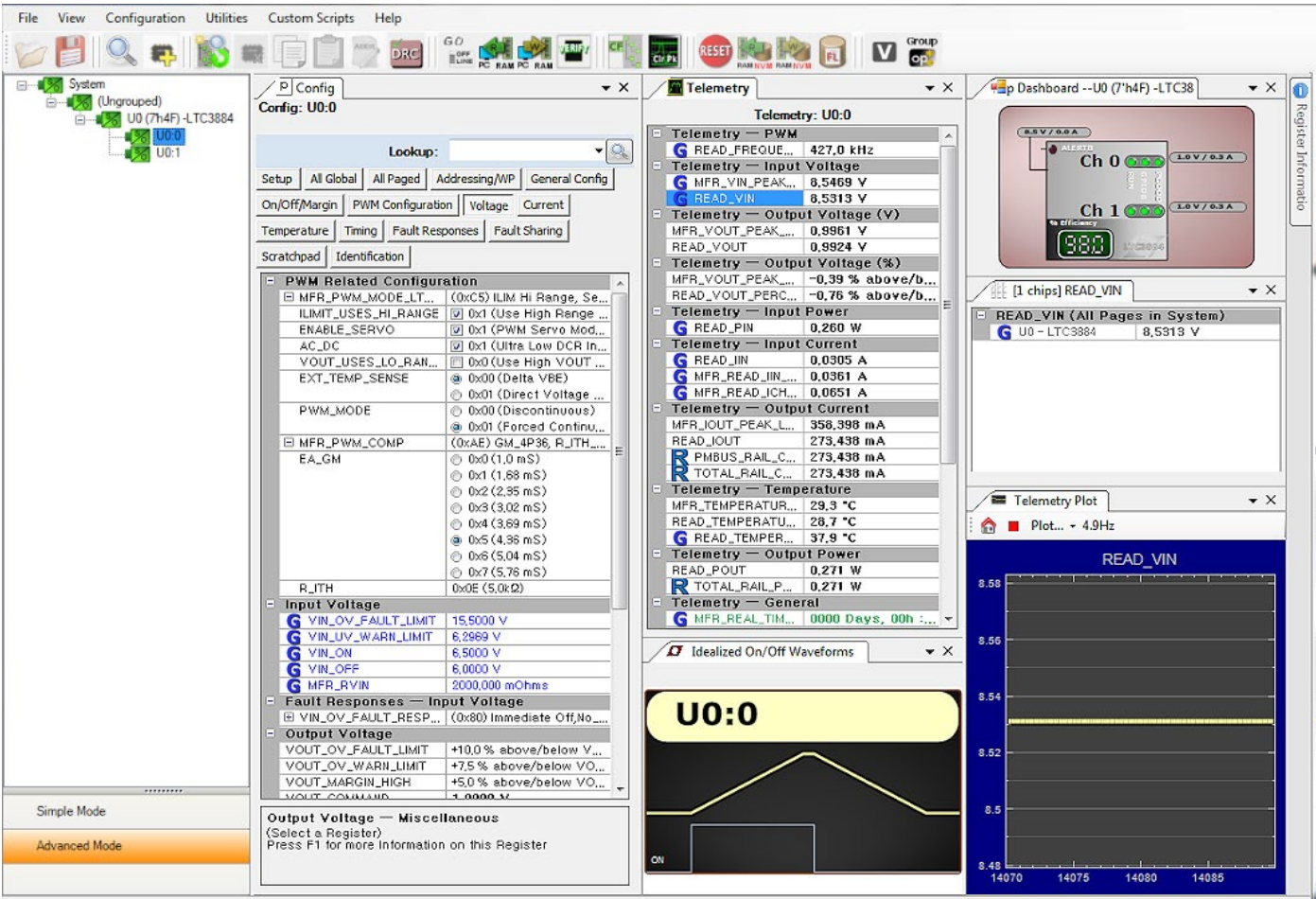
Figure 35. LTpowerPlay Screen Shot
