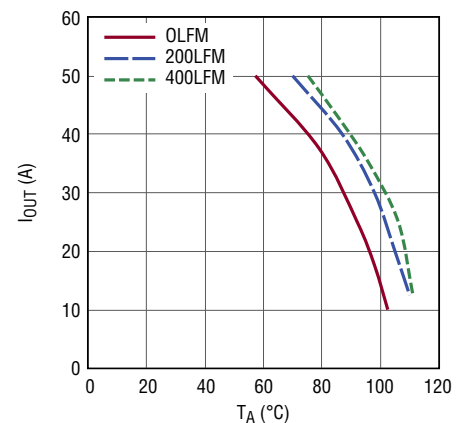
Figure 44. LTM4664A 54V IN 1.5V OUT 350kHz Derating Curve No Heat Sink
