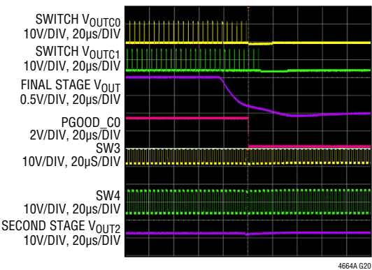
48V TO 1V AT 50A SHORTED LAST STAGE 1V OUTPUT VOUTC0 AND VOUTC1 IN PARALLEL
