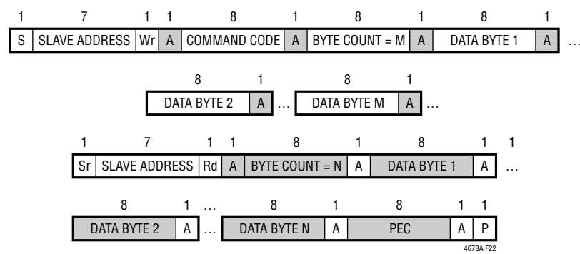
Figure 26. Block Write – Block Read Process Call with PEC
