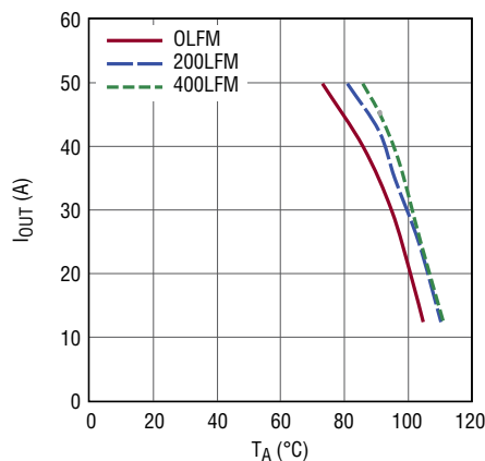
Figure 42. LTM4664A 54V IN 1V OUT Derating Curve No Heat Sink
