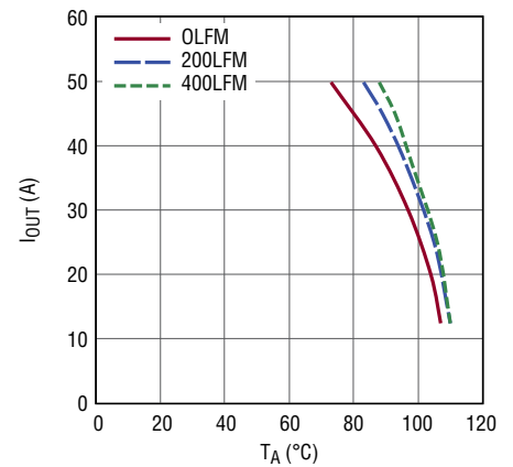
Figure 41. LTM4664A 48V IN 1V OUT Derating Curve No Heat Sink
