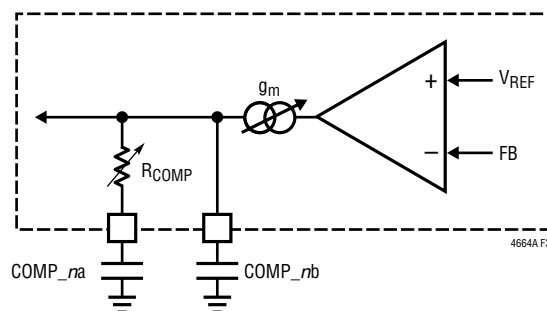
Figure 31. Programmable Loop Compensation
