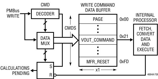
Figure 36. Write Command Data Processing
