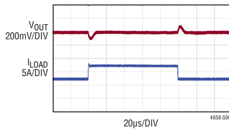
1.5V Output Transient Response, V IN = 3.3V
