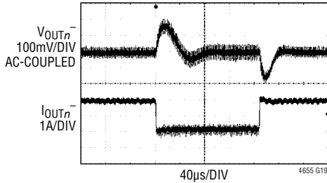
FIGURE 48 CIRCUIT, 24V IN . C_{INOUTn^-} = C_{INHn^-} = C_{DGNDn^-} = C_{Dn^-} = 4.7\mu\text{F} , C_{OUTn^-} = 47\mu\text{F} \times 2 , R_{ISETn^-} = 665\text{k}\Omega , R_{ISETn^-} = 100\text{k}\Omega , R_{PGDFBn^-} = 36.5\text{k}\Omega , R_{EXTVCCn^-} = 20\Omega , 1.8A TO 3.8A LOAD STEP AT 2A/µs
