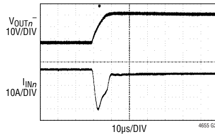
FIGURE 48 CIRCUIT, 19.2Ω LOAD PRIOR TO APPLICATION OF V_{OUTn^-} SHORT-CIRCUIT
