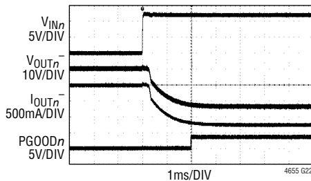
FIGURE 48 CIRCUIT, APPLICATION OF 12V IN , START-UP INTO 19.2Ω LOAD
