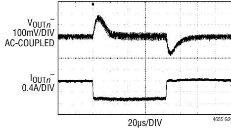
FIGURE 48 CIRCUIT, 0.625A TO 1.25A LOAD STEP AT 0.625A/µs
