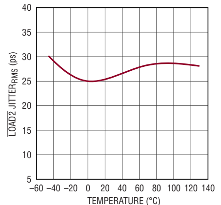
LOAD2 Jitter RMS vs Temperature
