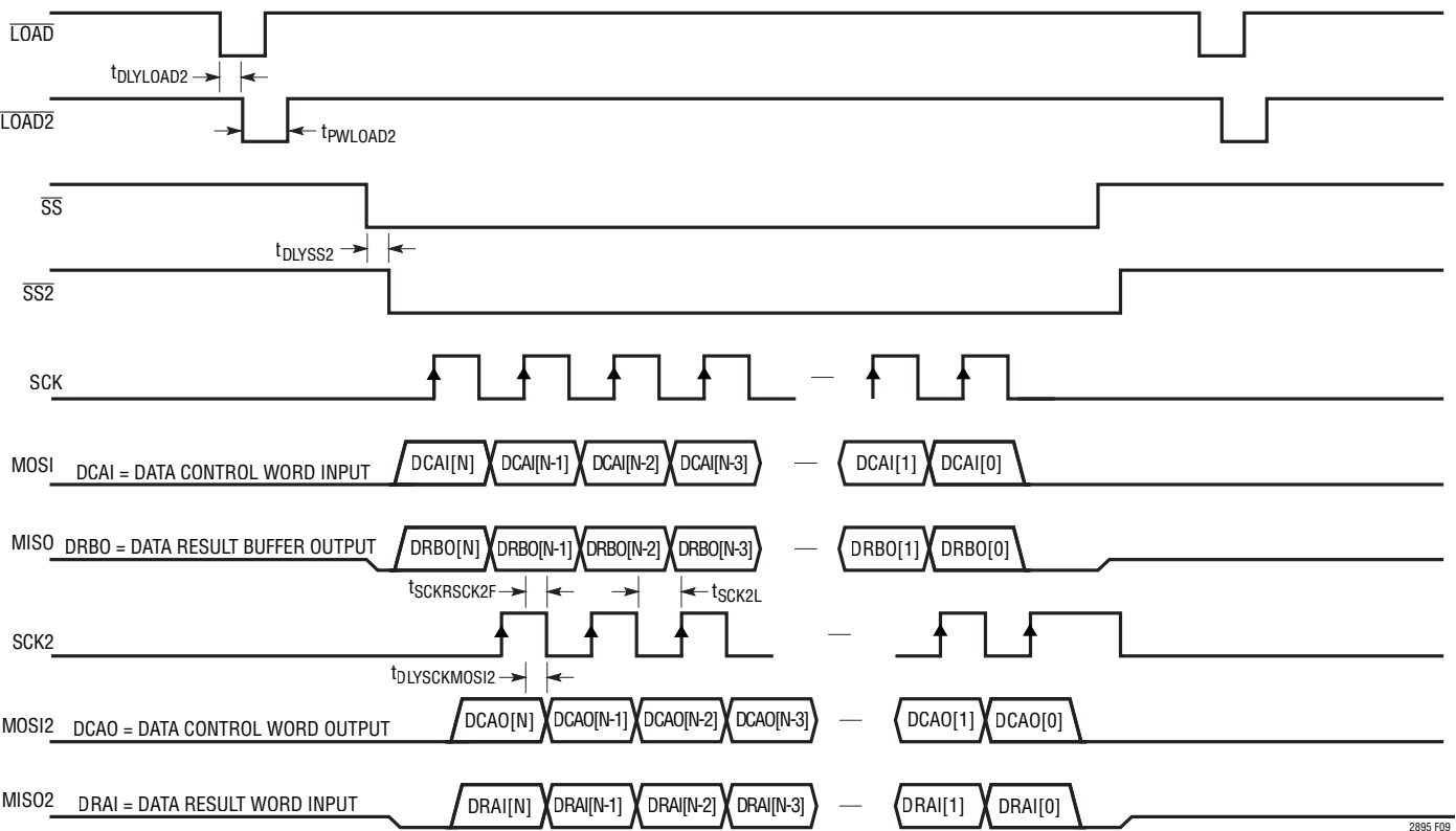
Figure 9. Logic and Isolated Side Interaction
