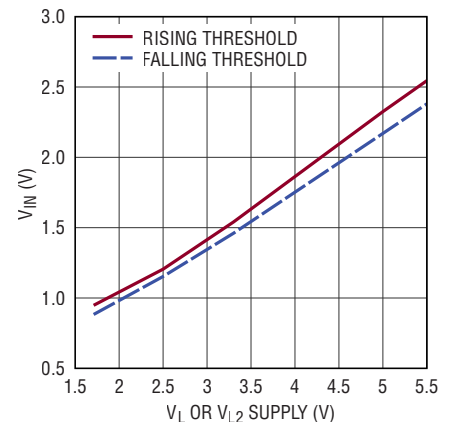
LOAD or MOSI, SCK, \overline{\text{SS}} , \overline{\text{SSB}} , MIS02 Inputs V_{IN} Thresholds vs V_L or V_{L2}
