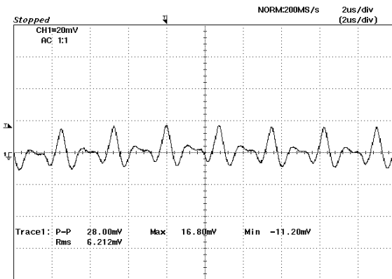
Figure 8: Output ripple & noise at 12Vin, 2.5V/6A out
