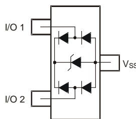
Device Schematic
