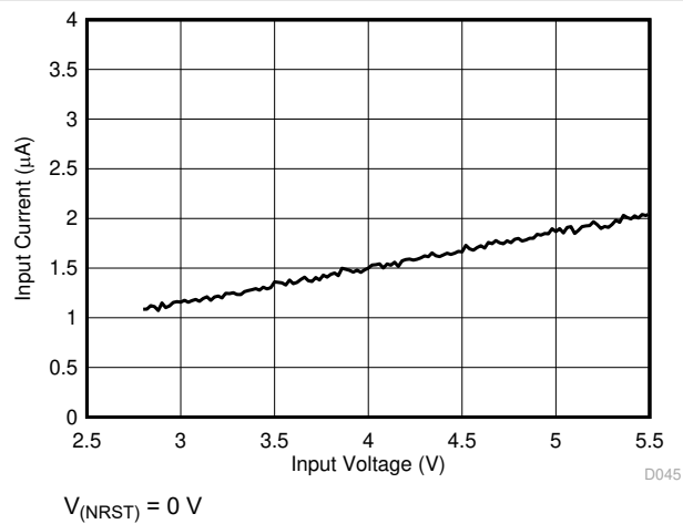
Figure 6-2. Shutdown Current Consumption vs Input Voltage
