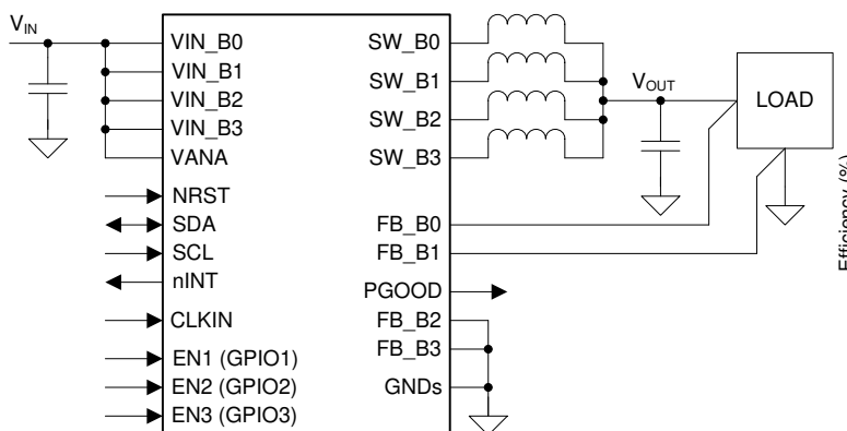
Simplified Schematic
