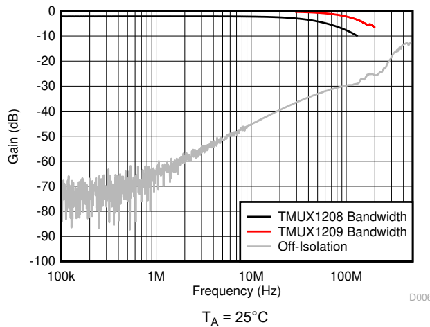
Figure 6-17. Frequency Response
