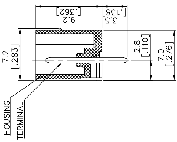
SECTION P-P
