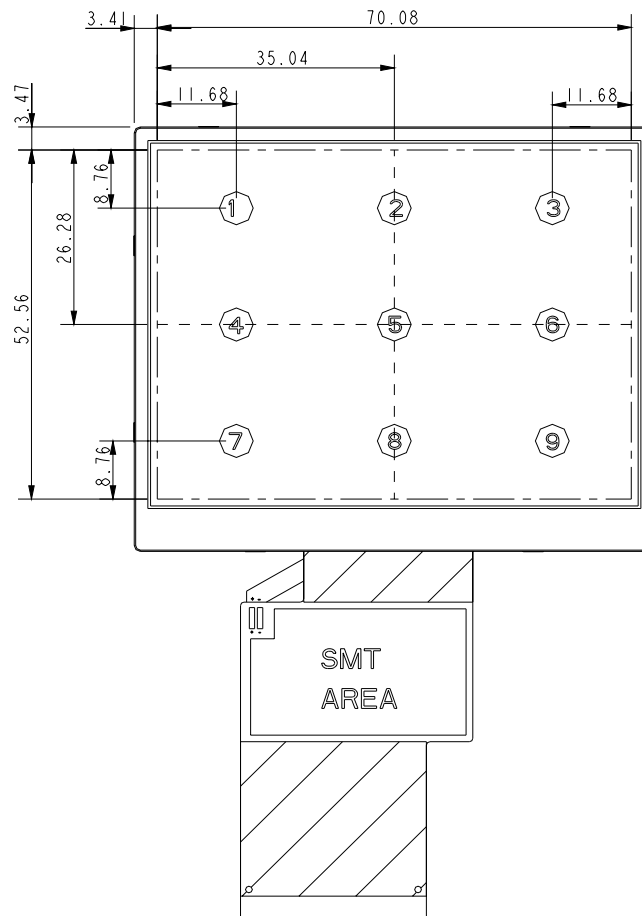
Fig.1 Measuring point
