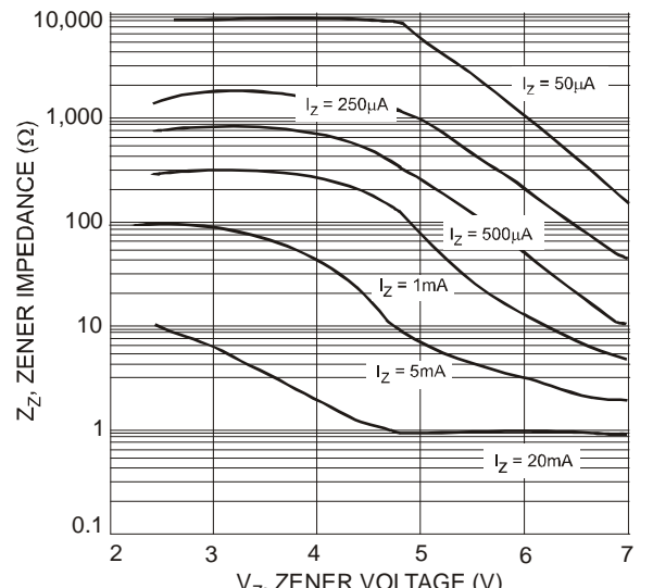
Fig. 11 Typical Zener Impedance Characteristics, DDZ9681 - DDZ9692
