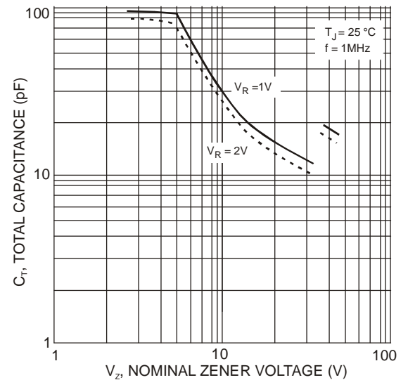
Fig. 10 Total Capacitance vs. Nominal Zener Voltage
