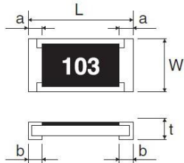
■MCR10/18/25/50/100
