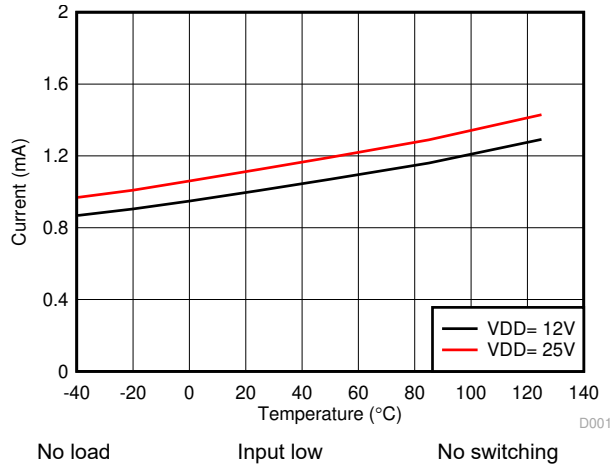
Figure 6-8. Per Channel ( I_{VDDA/B} ) Quiescent Supply Current vs Temperature
