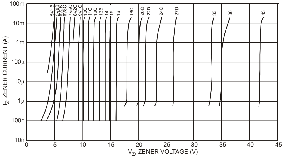
V Z , ZENER VOLTAGE (V) Fig. 3 Typical Zener Breakdown Characteristics
