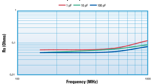
ESR vs Frequency DLI C17 AH Series
