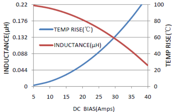
MWSA0618S-R22MT
