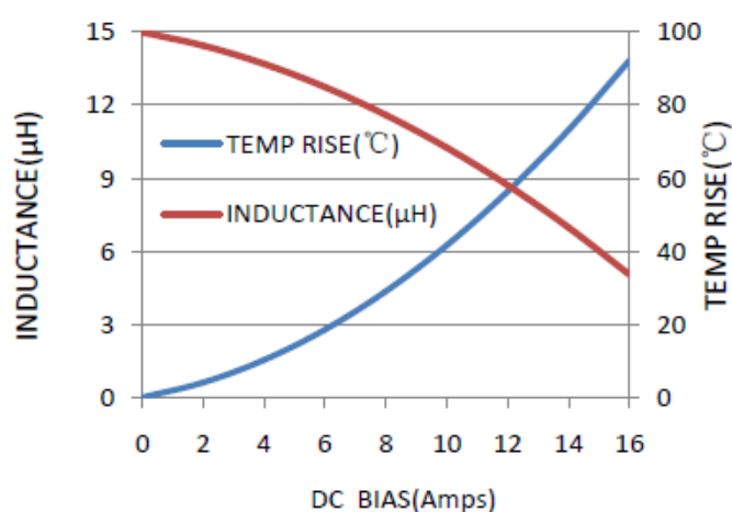
MWSA1206S-220MT
