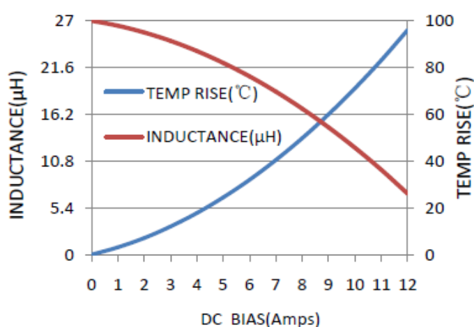
MWSA1206S-270MT
