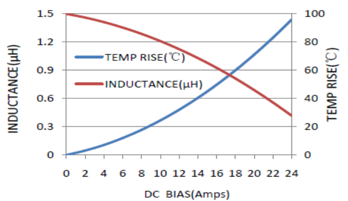
MWSA0603S-3R3MT
