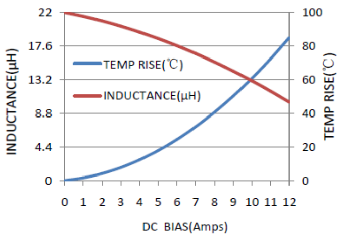
MWSA1206S-220MT
