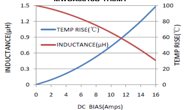
MWSA0518S-1R5MT
