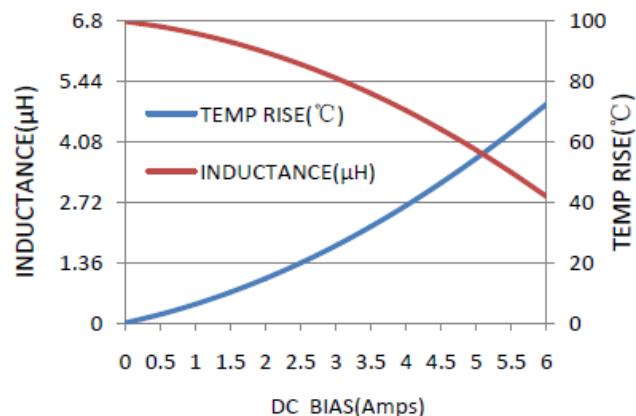
MWSA0503S-6R8MT
