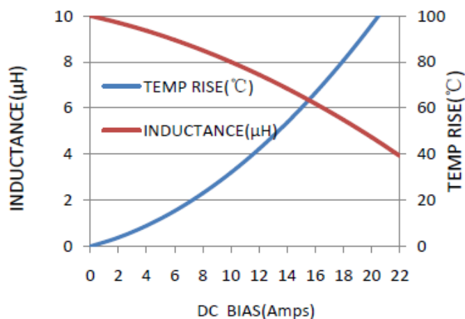
MWSA1206S-100MT
