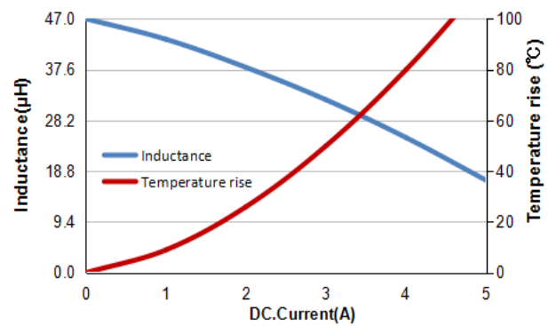
MWSA0605S-470MT
