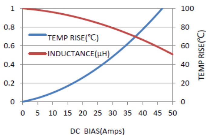
MWSA1204S-1R0MT
