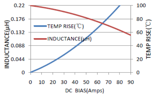
MWSA1004S-R22MT
