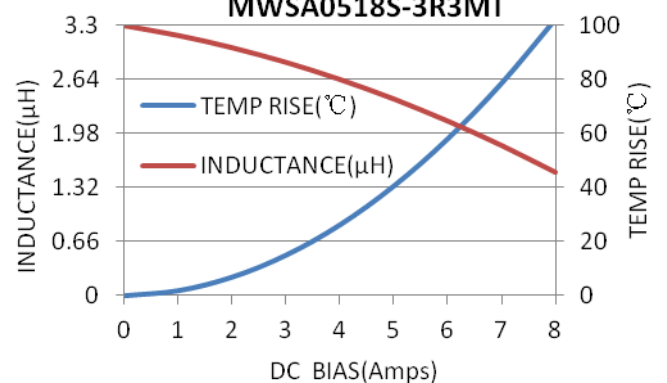
MWSA0518S-3R3MT
