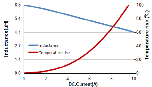
MWSA0605S-6R8MT
