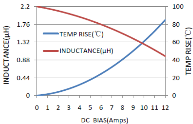
MWSA0503S-2R2MT
