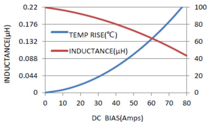
MWSA1204S-R22MT
