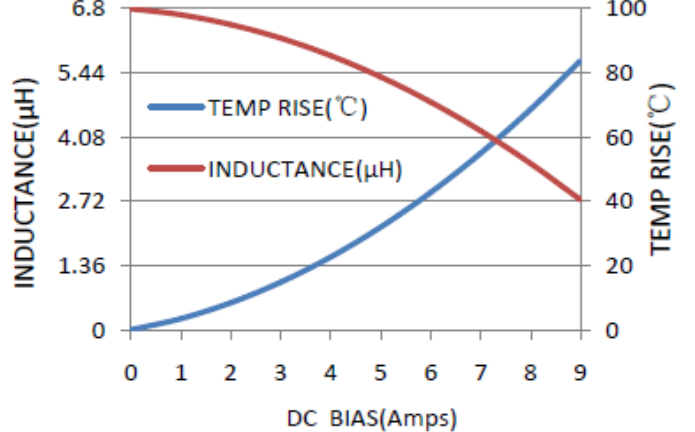
MWSA0603S-6R8MT
