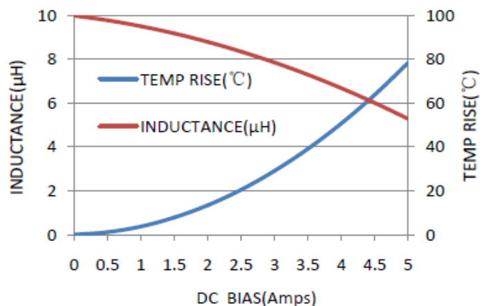
MWSA0503S-100MT
