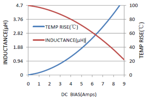
MWSA0503S-4R7MT
