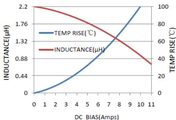
MWSA0518S-2R2MT
