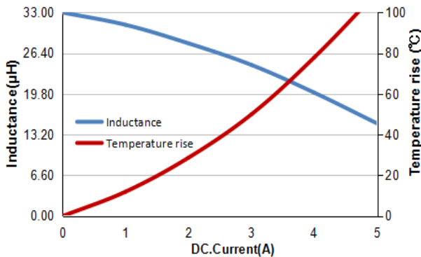
MWSA0605S-330MT
