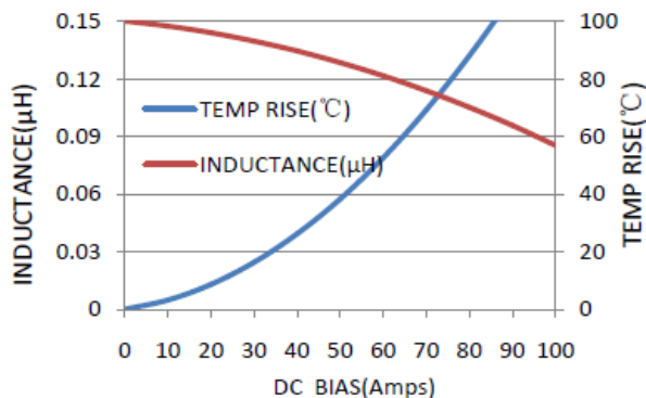
MWSA1004S-R15MT
