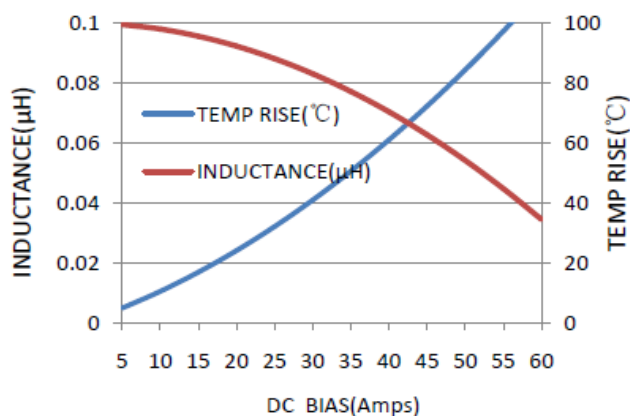
MWSA0618S-R10MT
