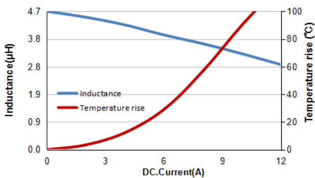
MWSA0605S-4R7MT
