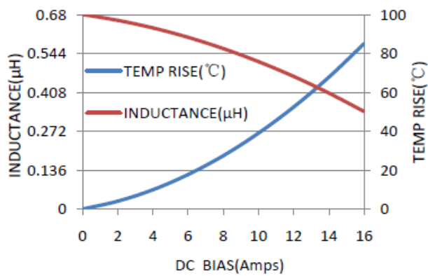
MWSA0503S-R68MT
