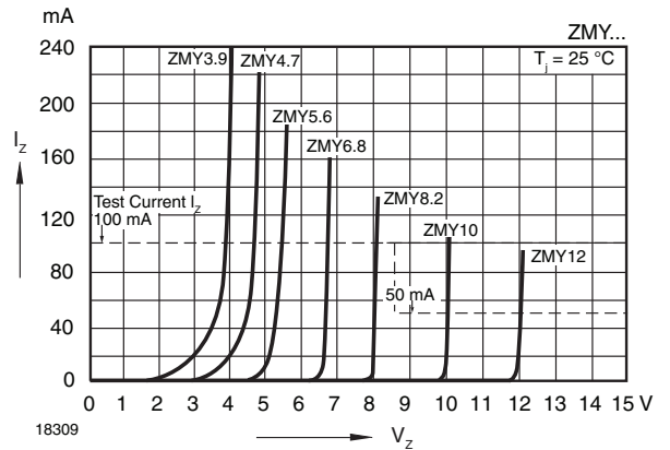
Fig. 5 - Breakdown Characteristics
