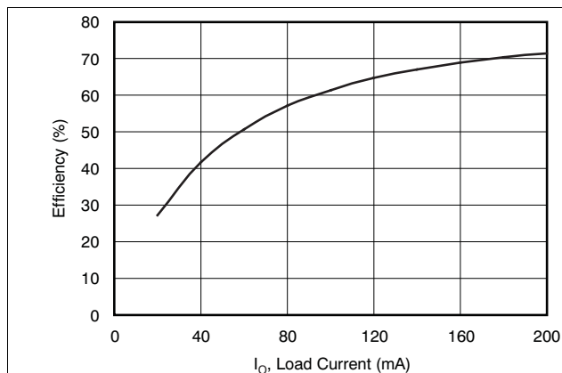
Figure 28. DCH010505S Efficiency
