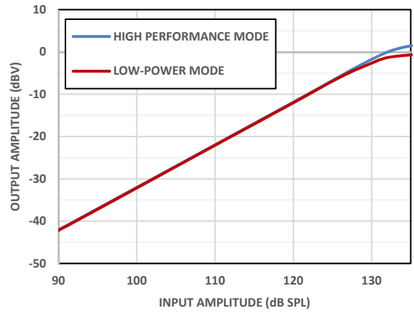
Figure 6. Linearity
