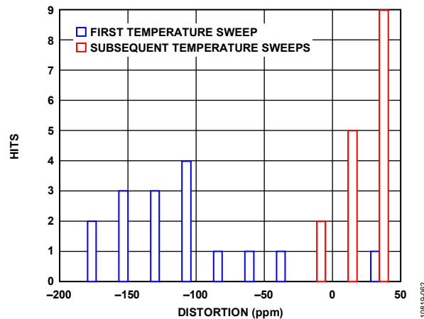
Figure 48. Thermal Hysteresis
