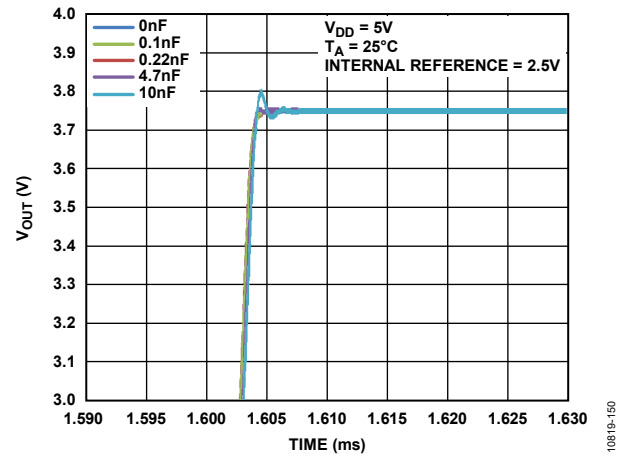
Figure 38. Settling Time at Various Capacitive Loads
