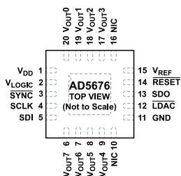
Figure 7. 20-Lead LFCSP Pin Configuration
